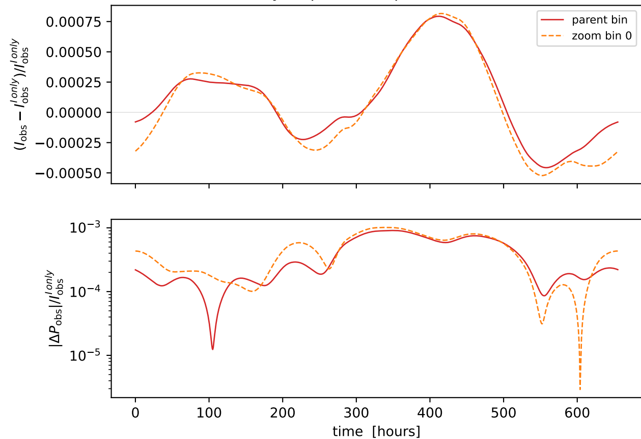
Polarized sky vs perfect depolarization at 50 MHz
