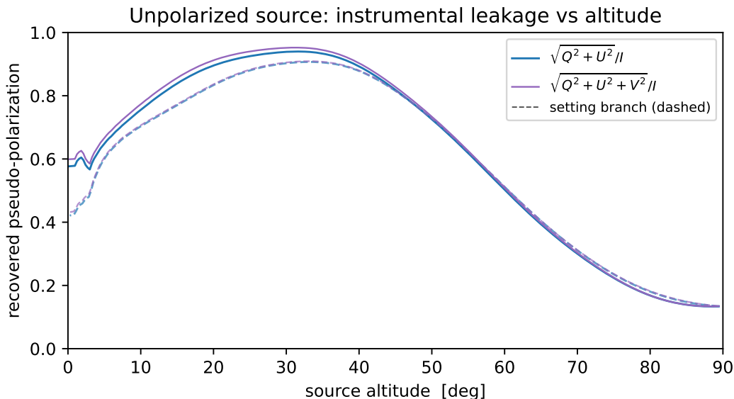
Figure 1: Unpolarized transiting source, raw X = E - W , Y = N - S polarimeter: the recovered pseudo-polarization is pure instrumental leakage (frequency-flat, so all channelizations coincide). Solid: rising branch, dashed: setting branch.
