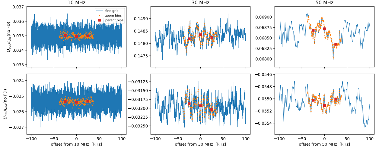
Figure 9: Beam-integrated Q_{\text{obs}}/I_{\text{obs}} (top) and U_{\text{obs}}/I_{\text{obs}} (bottom) across the \pm 100 kHz window at the time of maximum sky signal, for the three band centers (columns; each with its own calibrated weights), with the y-range zoomed onto the fine-grid structure (the Faraday-free level lies far off scale). The smooth mean level is almost entirely instrumental leakage of the unpolarized emission (Sec. 6); the fast “hash” riding on it, at the \text{few} \times 10^{-3} relative level, is the surviving sky polarization scrambled by the many rotation measures within the beam. The frequency scale of the hash stretches as \nu^3 : at 10 MHz it is unresolved on this plot, at 30 MHz it is a dense stipple, while at 50 MHz the fine grid (blue) visibly resolves the individual Faraday oscillations of the dominant rotation measures, with coherence lengths of tens of kHz. Correspondingly, the zoom bins trace a smoothed version of the hash and the parent bins average over it at 10–30 MHz, but at 50 MHz even the 25 kHz parent bins begin to follow the true spectral structure.
