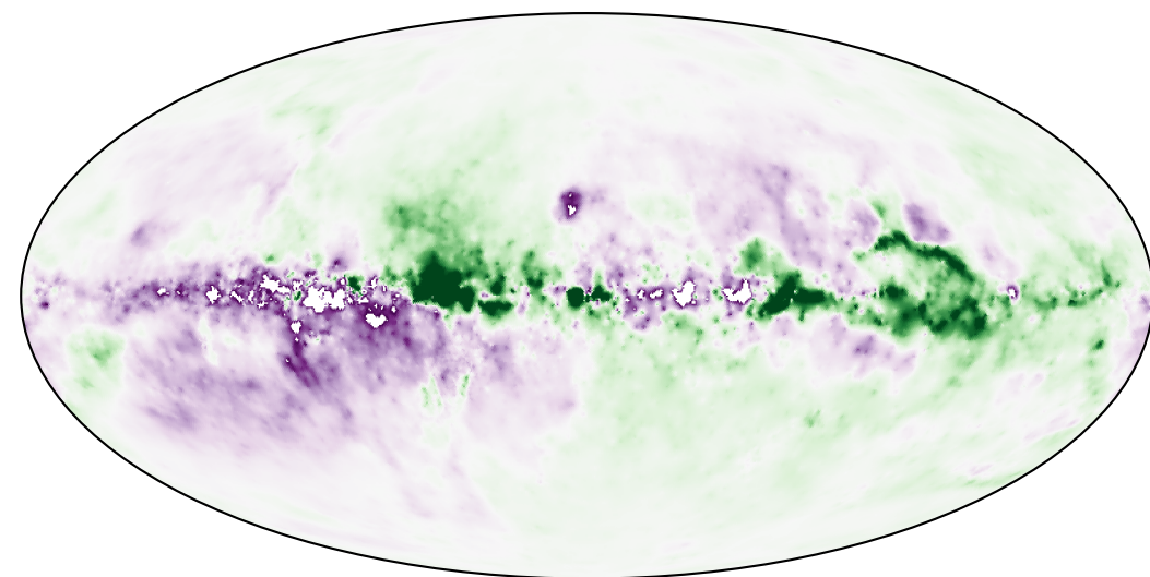
Rotation Measure
