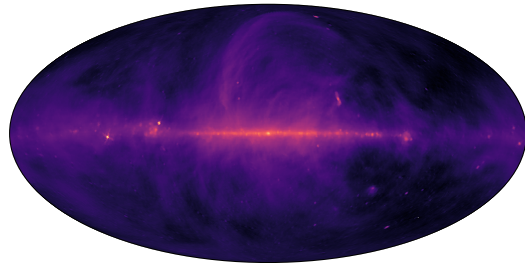
Intrinsic Stokes I
