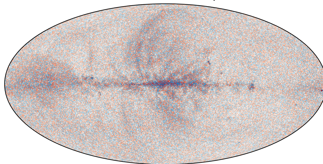
Rotated Stokes Q
