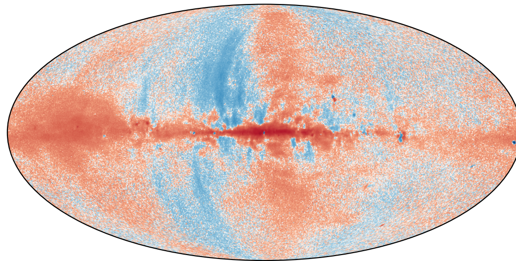
Intrinsic Stokes Q
