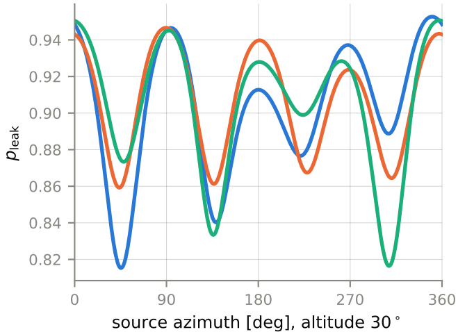
(b) azimuthal structure (C4 test)
