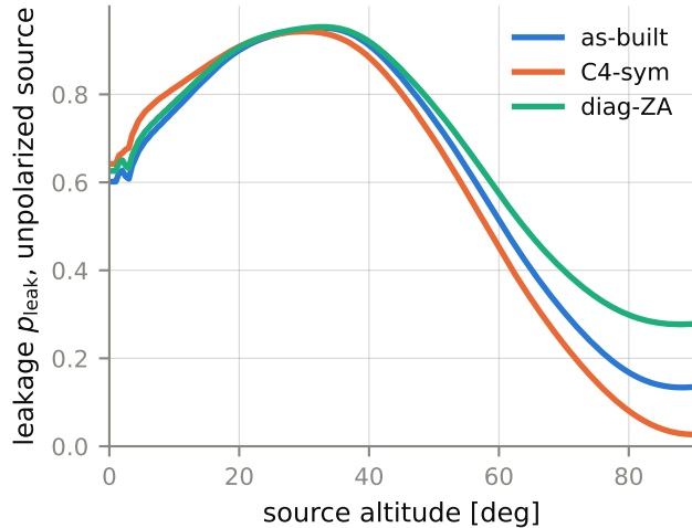
(a) naive polarimeter, az=0^\circ
