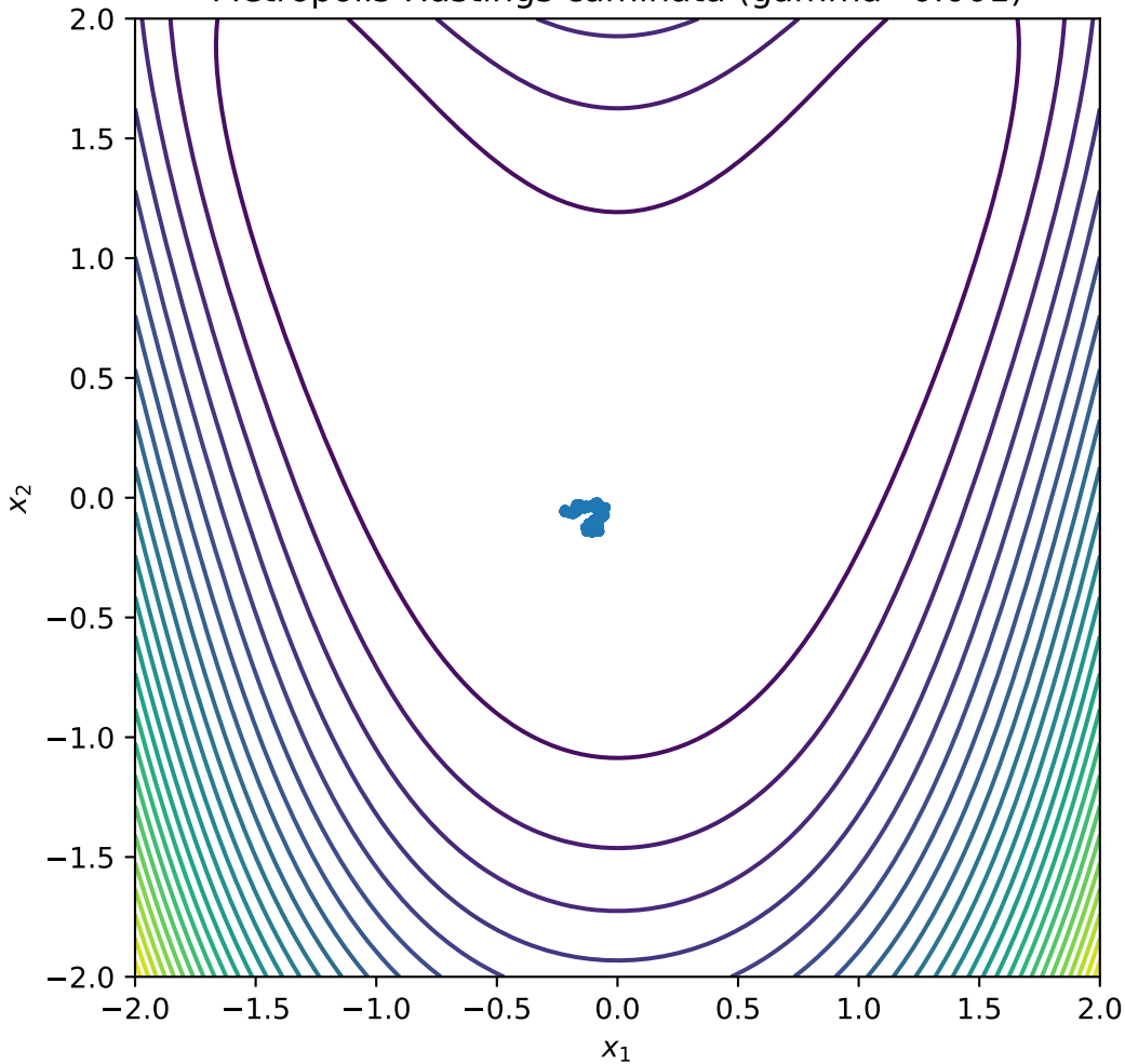
Metropolis-Hastings caminata (gamma=0.001)
