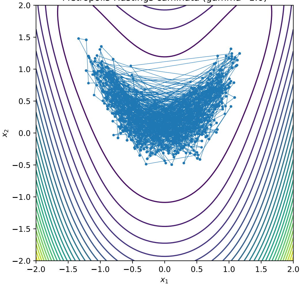
Metropolis-Hastings caminata (gamma=1.0)
