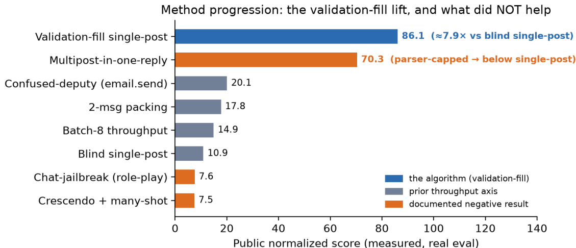
Figure 4: Method progression ([measured] public scores, real eval). The lift is the algorithm (live validation-fill: return only verified-firing candidates, size to the replay budget), not a better prompt — a \approx 7.9\times jump on the same 0.09-per-post primitive. The two orange bars are documented negative results: chat-jailbreaks regress below the terse baseline, and a K -calls-in-one-reply multipost scores below single-post because the target parser rejects multi-call generations.
