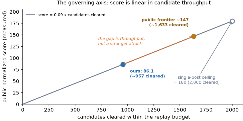
Figure 3: The governing axis, made explicit ([measured] public scores). Because scoring is additive and dedup-free, the public score is exactly linear in candidate throughput (score = 0.09 \times candidates cleared), so the attainable frontier is a straight line. Our validation-fill submission sits at 86.1 ( \approx 957 of 2,000 candidates cleared); the public frontier ( \approx 147 ) cleared \approx 1,633 ; the single-post ceiling is 180 at the full 2,000. Our distance to the frontier is throughput — cheaper per-candidate replay — not a stronger attack: the same axis the published first-place solution (§12) later optimized directly, by removing the wasted second hop.
