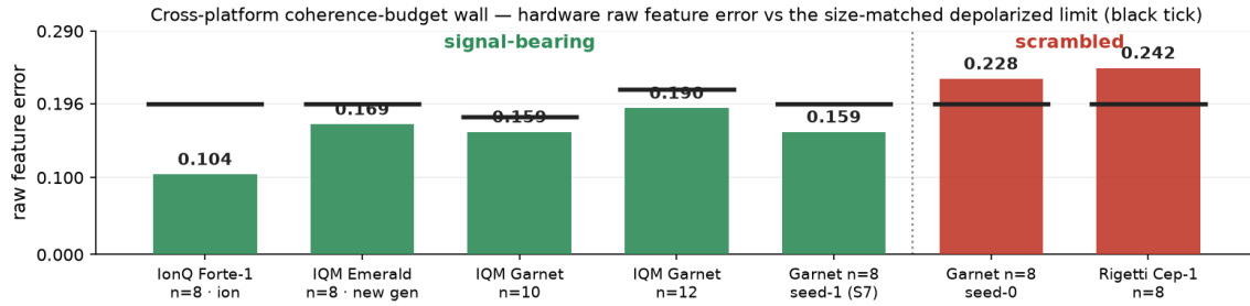
Figure 3. Cross-platform coherence-budget wall: mean raw feature error vs the size-matched depolarized limit (black ticks; 4k shots, IonQ 500).
