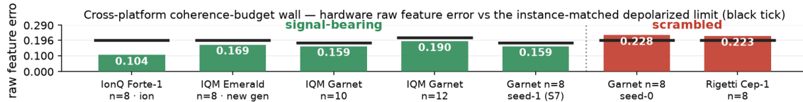
Figure 3. Cross-platform coherence-budget wall: mean raw feature error vs the instance-matched depolarized limit \text{mean}|F_{\text{exact}}| (black ticks; 4k shots, IonQ 500). Five configs signal-bearing, two scrambled. The adjacent Garnet n=8 seed-1 (0.159) vs seed-0 (0.228) pair — same chip and session — refutes a size law. Seed-0 limits 0.196/0.179/0.214; seed-1 carries its own 0.1806 (§6).
