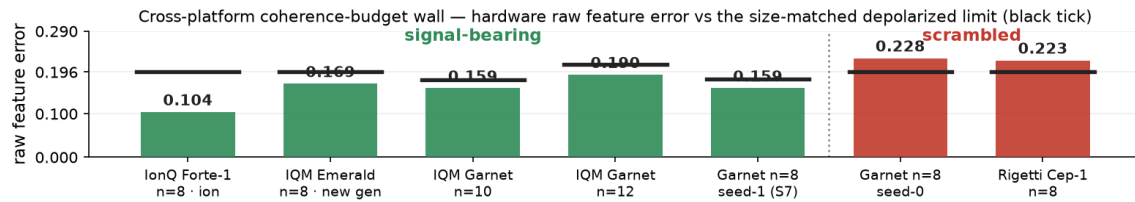
Figure 3. Cross-platform coherence-budget wall: mean raw feature error vs the instance-matched depolarized limit mean |F_{\text{exact}}| (black ticks; 4k shots, IonQ 500). Five configs are signal-bearing (below the limit), two scrambled (Garnet n=8 seed-0 0.228; Rigetti 0.223). The adjacent Garnet n=8 seed-1 (0.159) vs seed-0 (0.228) pair — same chip and session — refutes a size law. Seed-0 limits 0.196/0.179/0.214 at n=8/10/12; seed-1 carries its own 0.1806 — verdict unchanged (§6).
