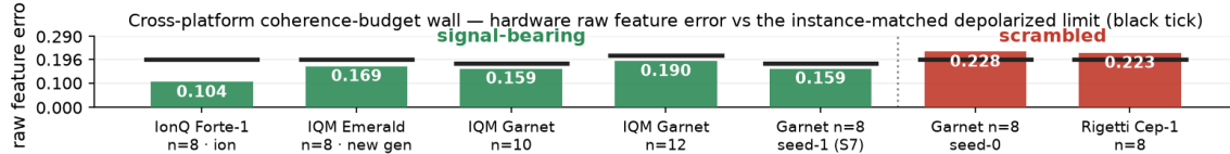
Figure 3. Cross-platform coherence-budget wall: mean raw feature error vs the instance-matched depolarized limit \text{mean}|F_{\text{exact}}| (black ticks; 4k shots, IonQ 500). Five configs signal-bearing, two scrambled. The adjacent Garnet n=8 seed-1 (0.159) vs seed-0 (0.228) pair — same chip and session — refutes a size law. Seed-0 limits 0.196/0.179/0.214; seed-1 carries its own 0.1806 (§6).
