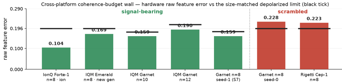
Figure 3. Cross-platform coherence-budget wall: mean raw feature error vs the instance-matched depolarized limit \text{mean}|F_{\text{exact}}| (black ticks; 4k shots, IonQ 500). Five configs are signal-bearing (below the limit), two scrambled (Garnet n=8 seed-0 0.228; Rigetti 0.223). The adjacent Garnet n=8 seed-1 (0.159) vs seed-0 (0.228) pair — same chip, same session — refutes a size law: the n=8 scrambling is specific to the seed-0 instance. Seed-0 limits 0.196/0.179/0.214 at n=8/10/12; seed-1 carries its own 0.1806 (n=8) — verdict unchanged (§6).
