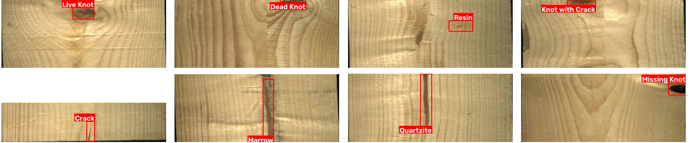
Figure 2: Examples of the eight defect classes annotated in the wood dataset (Nomihisa, 2024): Live Knot, Dead Knot, Resin, Knot with Crack, Crack, Marrow, Quartzite, and Missing Knot (left to right, top to bottom).
