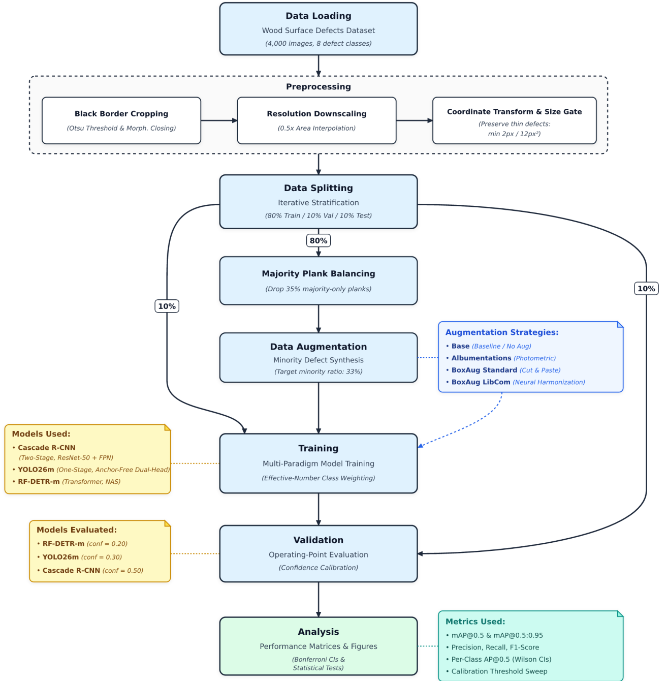
Figure 3: Overview of the proposed five-stage experimental pipeline for timber defect detection benchmarking.
