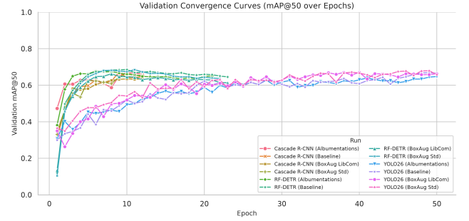
Figure 11: mAP@0.5 validation convergence curves during training.
