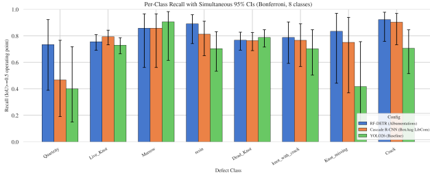
Figure 9: Per-class recall with simultaneous 95% family-wise confidence intervals for the best configuration of each paradigm. Error bars are 99.375% Wilson intervals per class, i.e. simultaneous 95% family-wise coverage over the 8 classes (Bonferroni).
