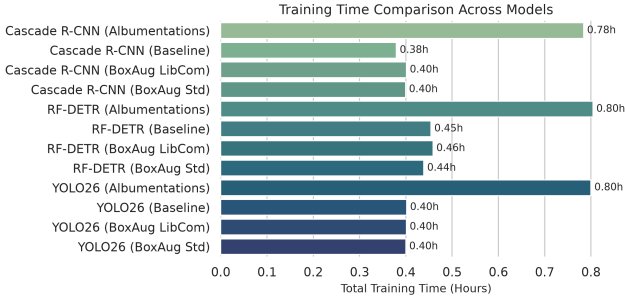
Figure 13: Comparison of total training time per configuration.
