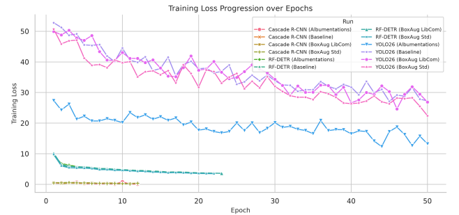
Figure 12: Training loss progression over epochs for all 12 configurations.
