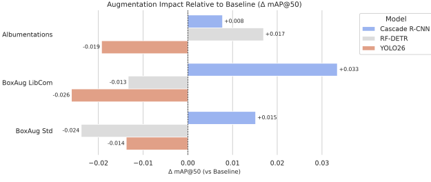
Figure 6: Impact of augmentation strategies relative to baseline ( \Delta mAP@0.5).
