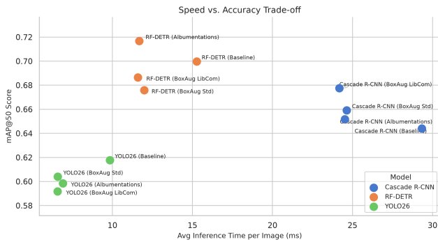
Figure 10: Trade-off between inference speed (ms/image) and precision (mAP@0.5).
