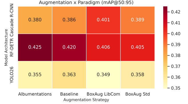
Figure 5: mAP@0.5:0.95 performance matrix for the same 12 configurations.
