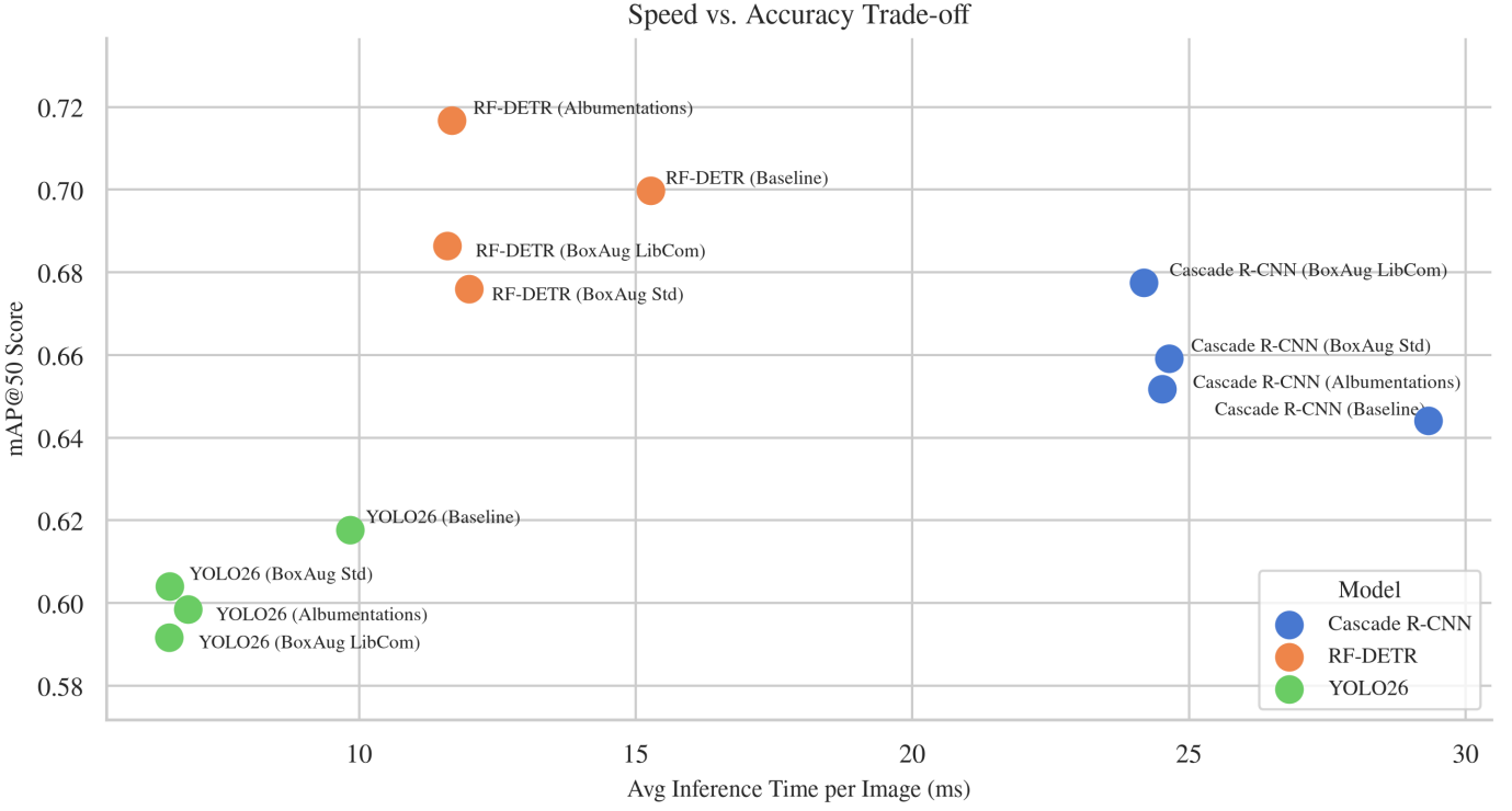
Figure 11: Trade-off between inference speed (ms/image) and precision (mAP@0.5).
