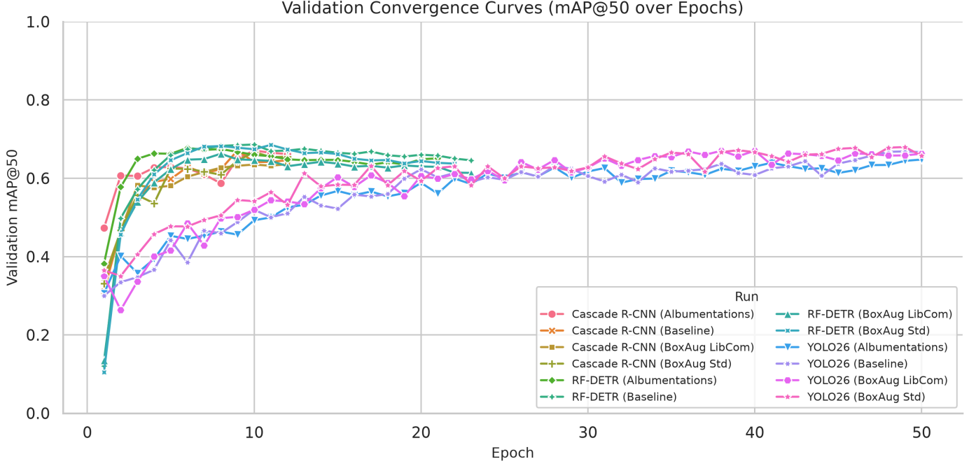
Figure 15: mAP@0.5 validation convergence curves during training.
