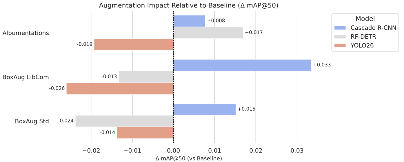
Figure 7: Impact of augmentation strategies relative to baseline ( \Delta mAP@0.5).
