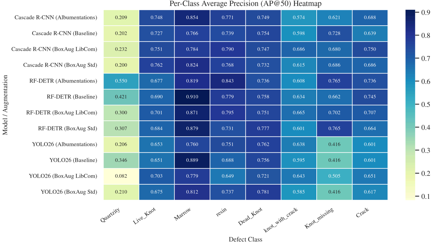
Figure 8: Heatmap of average precision per defect class (AP@0.5).
