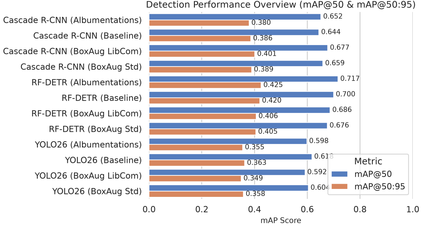
Figure 6: Overview of mAP@0.5 and mAP@0.5:0.95 per model-augmentation configuration, confirming the RF-DETR, Cascade R-CNN, YOLO26 order under both metrics.
