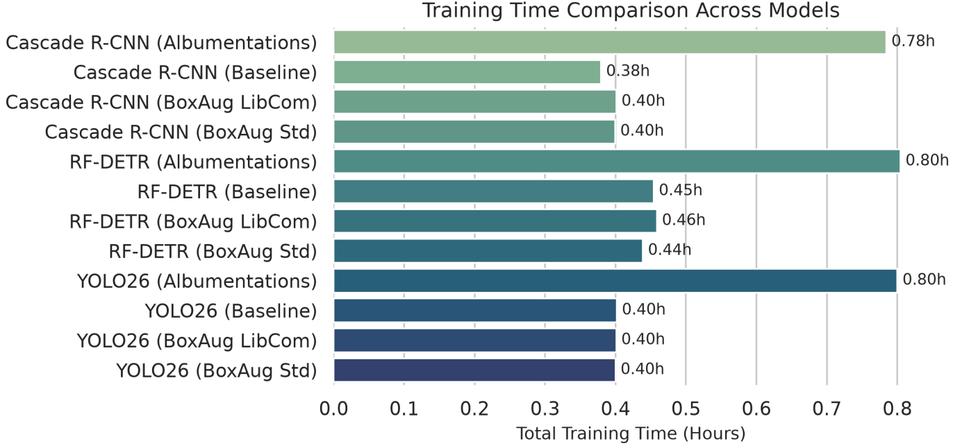
Figure 17: Comparison of total training time per configuration.
