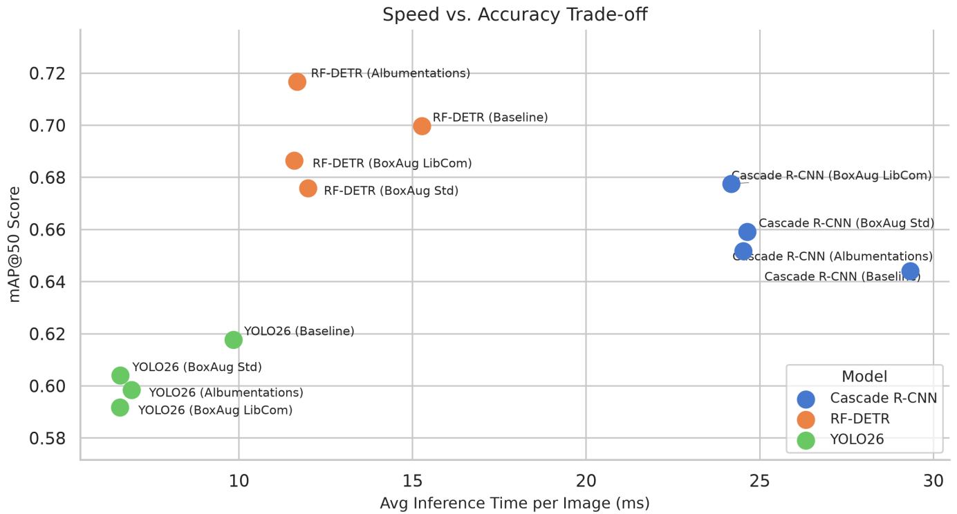
Figure 13: Trade-off between inference speed (ms/image) and precision (mAP@0.5).
