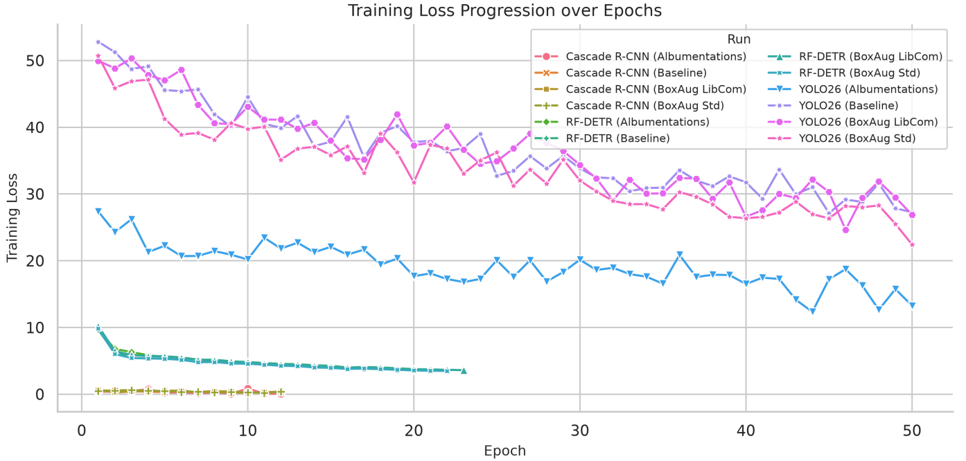
Figure 16: Training loss progression over epochs for all 12 configurations.
