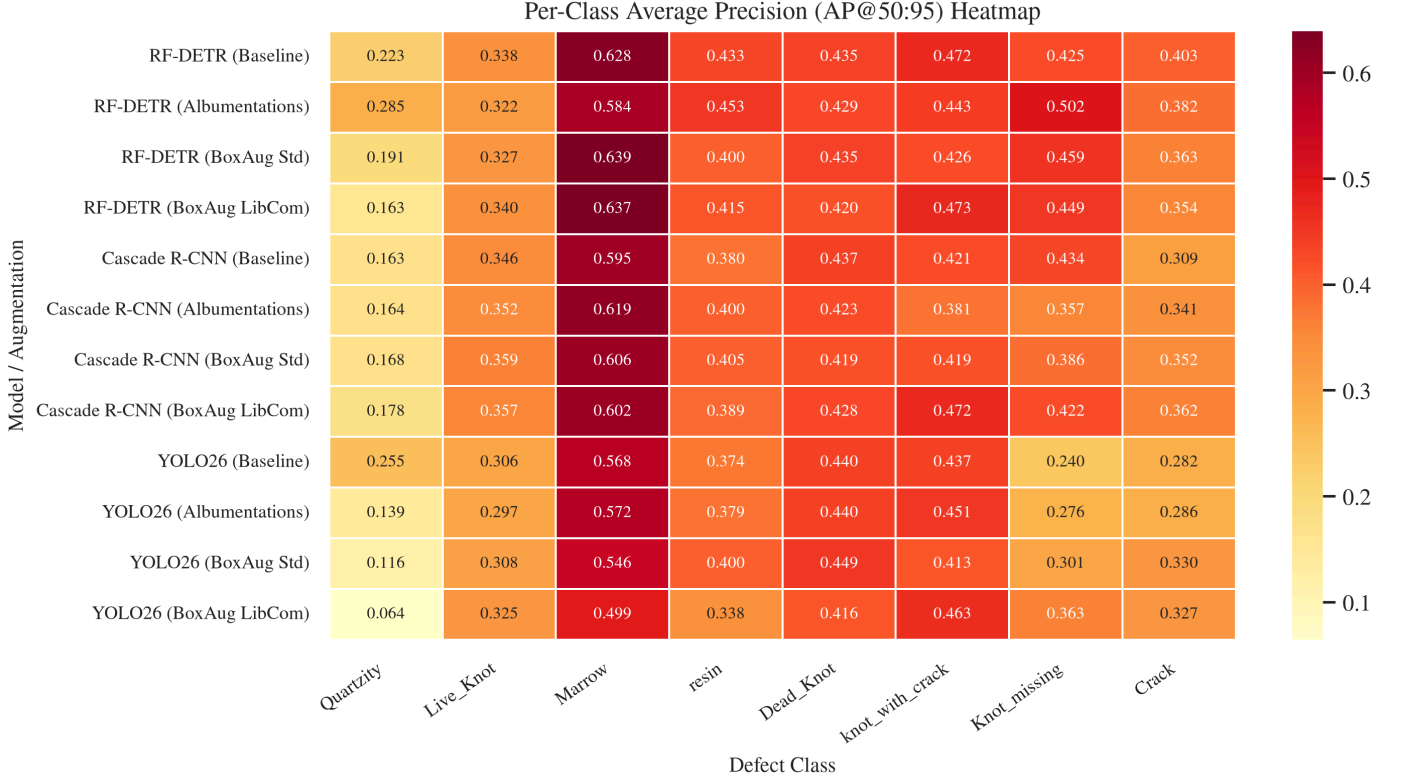
Figure 10: Heatmap of average precision per defect class (AP@0.5:0.95).
