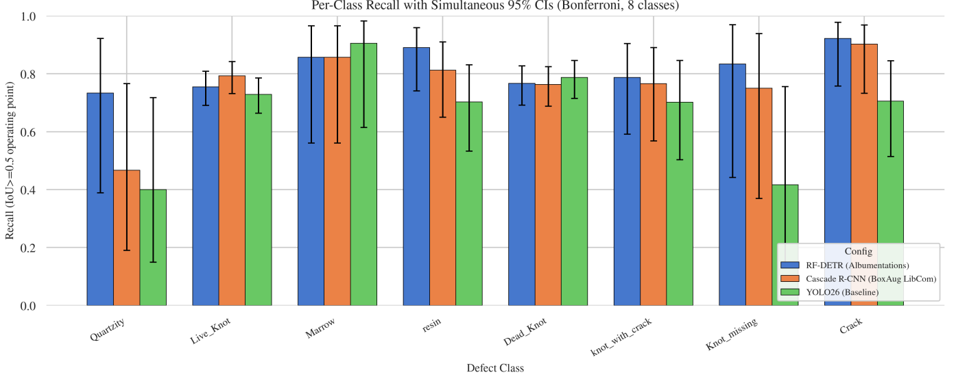
Figure 11: Per-class recall with simultaneous 95% family-wise confidence intervals for the best configuration of each paradigm. Error bars are 99.375% Wilson intervals per class, i.e. simultaneous 95% family-wise coverage over the 8 classes (Bonferroni).
