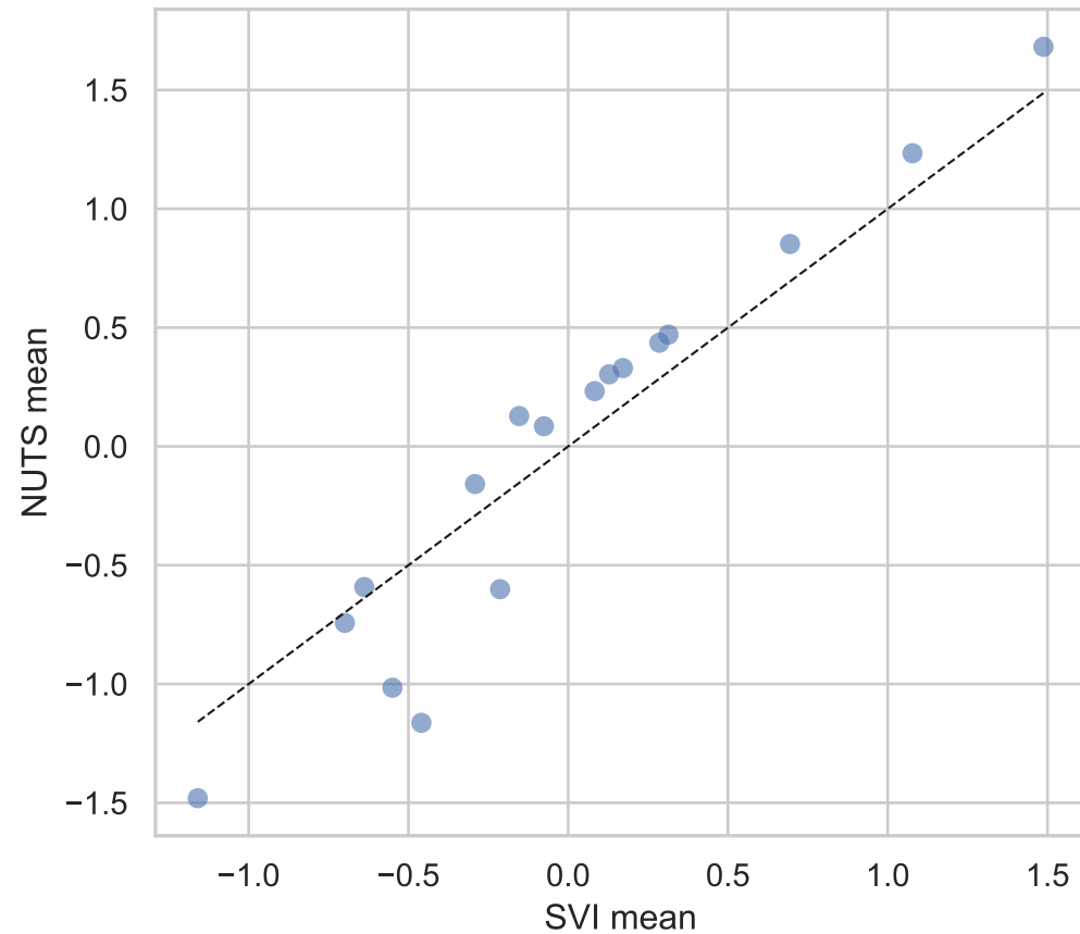
Constructors ( \tau = 0.882 )
