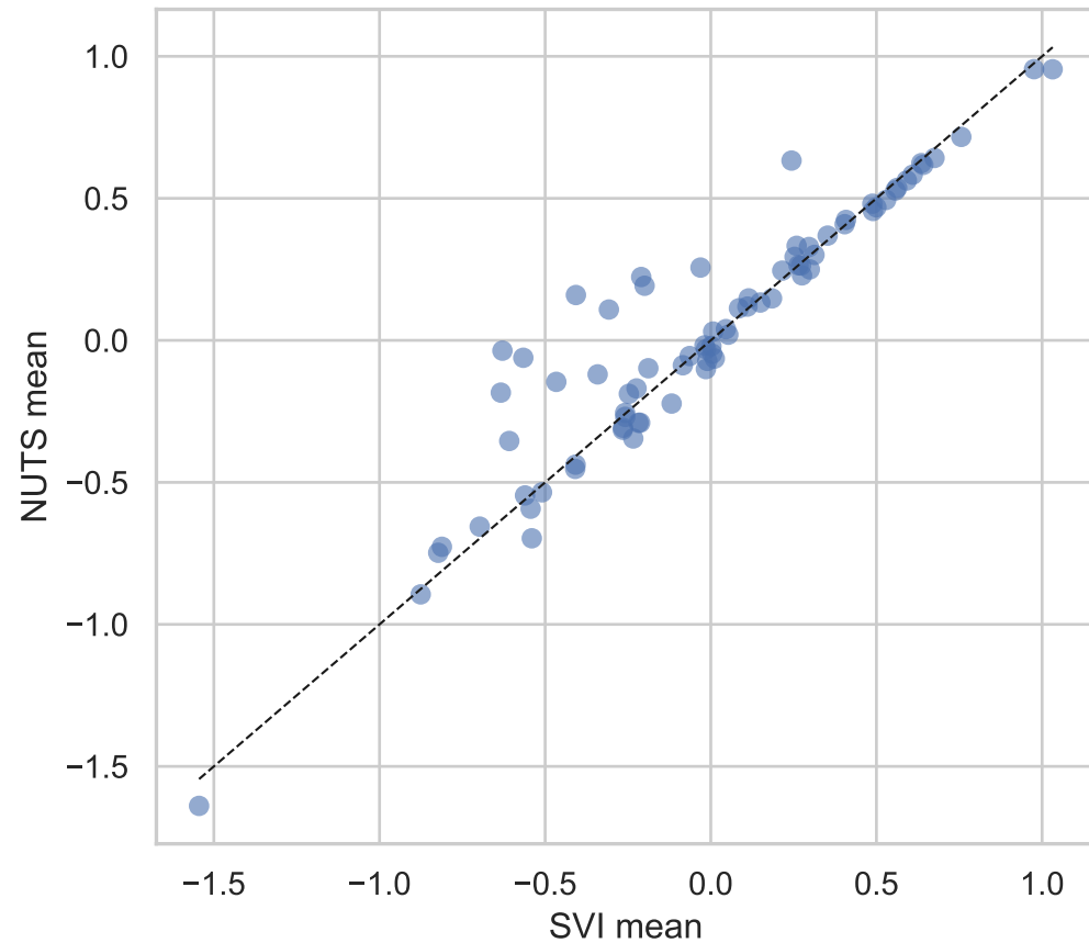
Drivers ( \tau = 0.802 )
