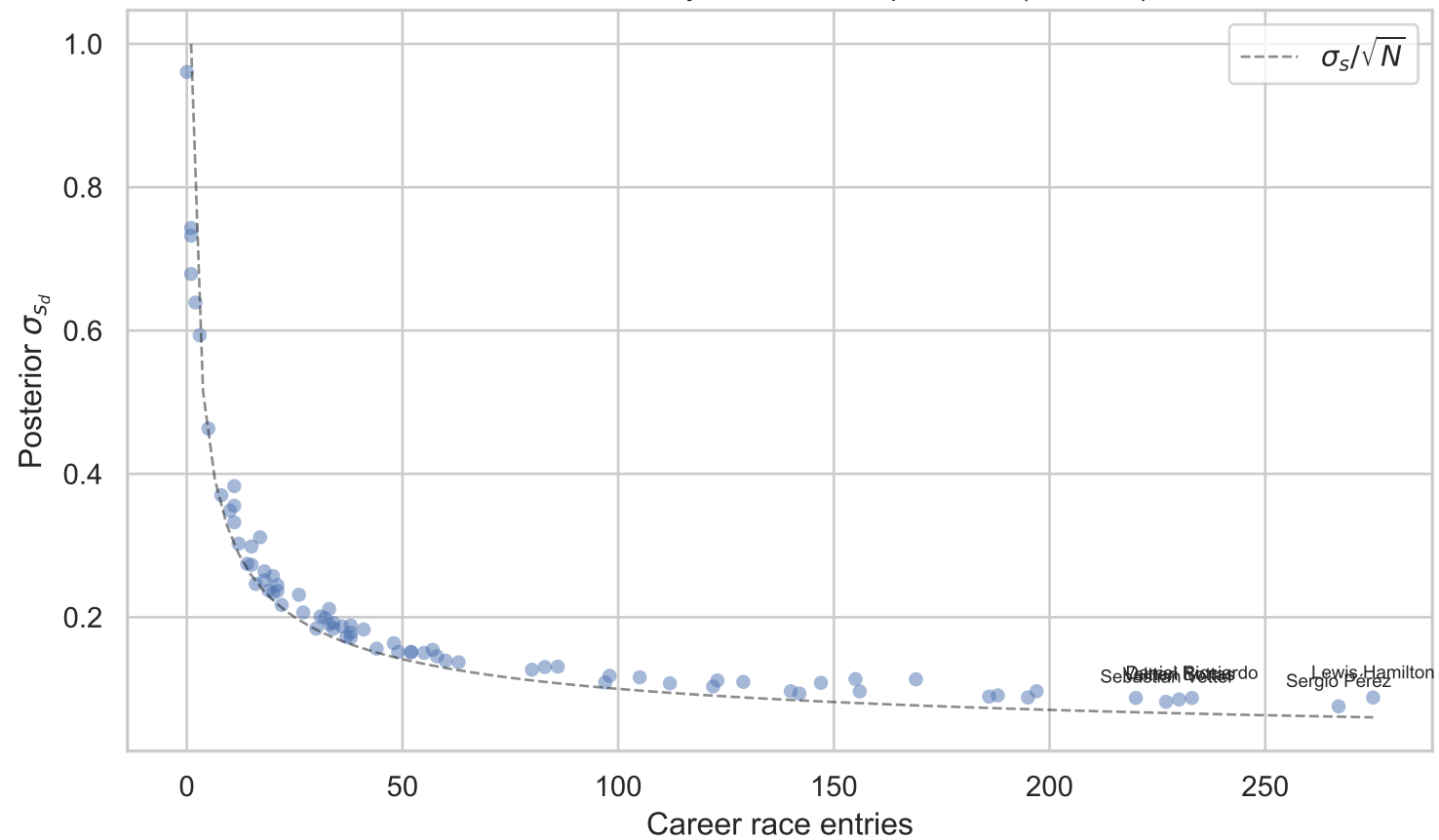
Posterior Uncertainty vs Career Experience (Model 1)
