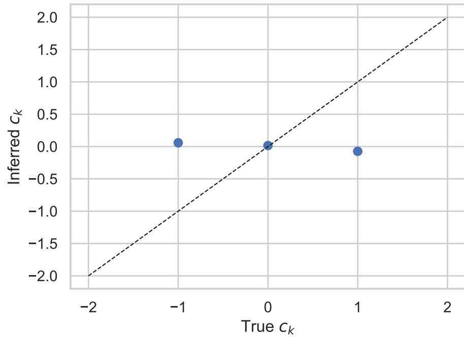
Constructors ( \tau = -1.000 )
