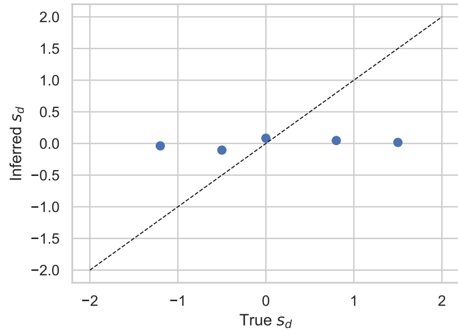
Drivers ( \tau = 0.200 )
