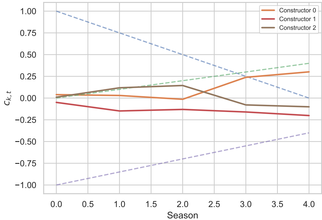
Constructor AR(1) Recovery
