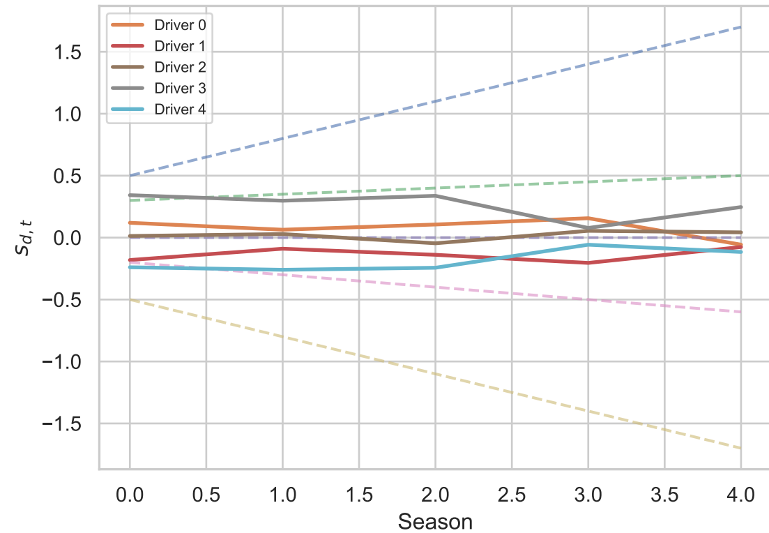
Driver AR(1) Recovery
