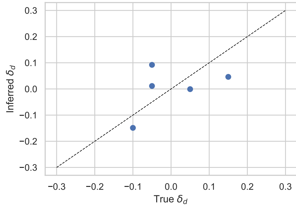
\delta_d Recovery
