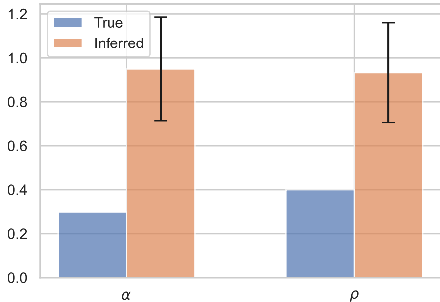
\alpha/\rho Recovery
