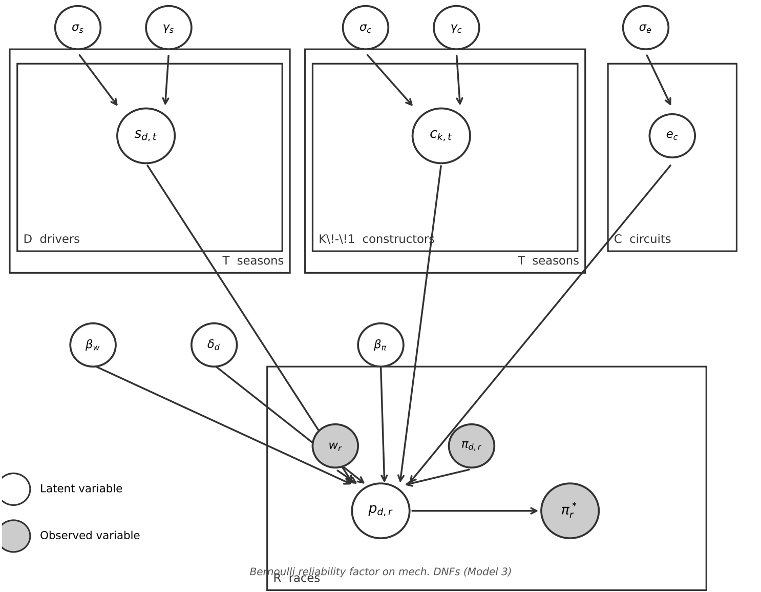
Generative Model — Plate Notation (Model 3, Full)
