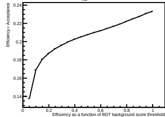
16 < p_{T,D^0} < 20 \text{ GeV/c}
