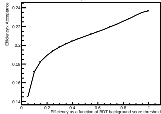
12 < p_{T,D^0} < 16 \text{ GeV/c}
