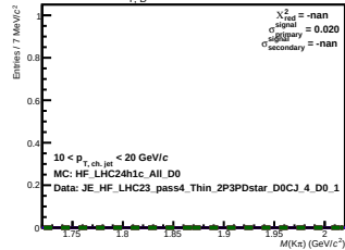
8 < p_{T, D^0} < 10 \text{ GeV}/c
