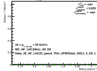
7 < p_{T, D^0} < 8 \text{ GeV}/c
