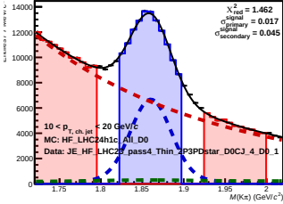
10 < p_{T, D^0} < 12 \text{ GeV}/c
