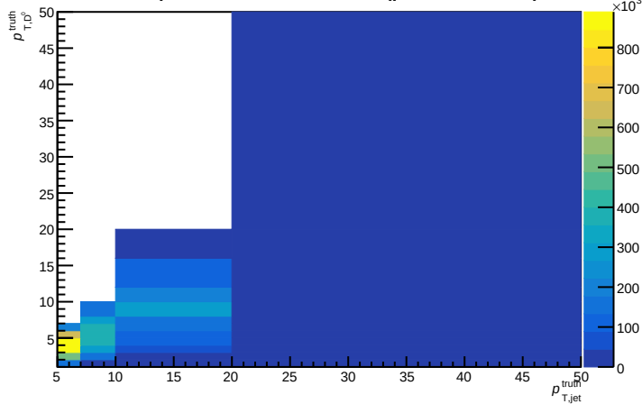
Prompt D 0 's denominator (particle level)
