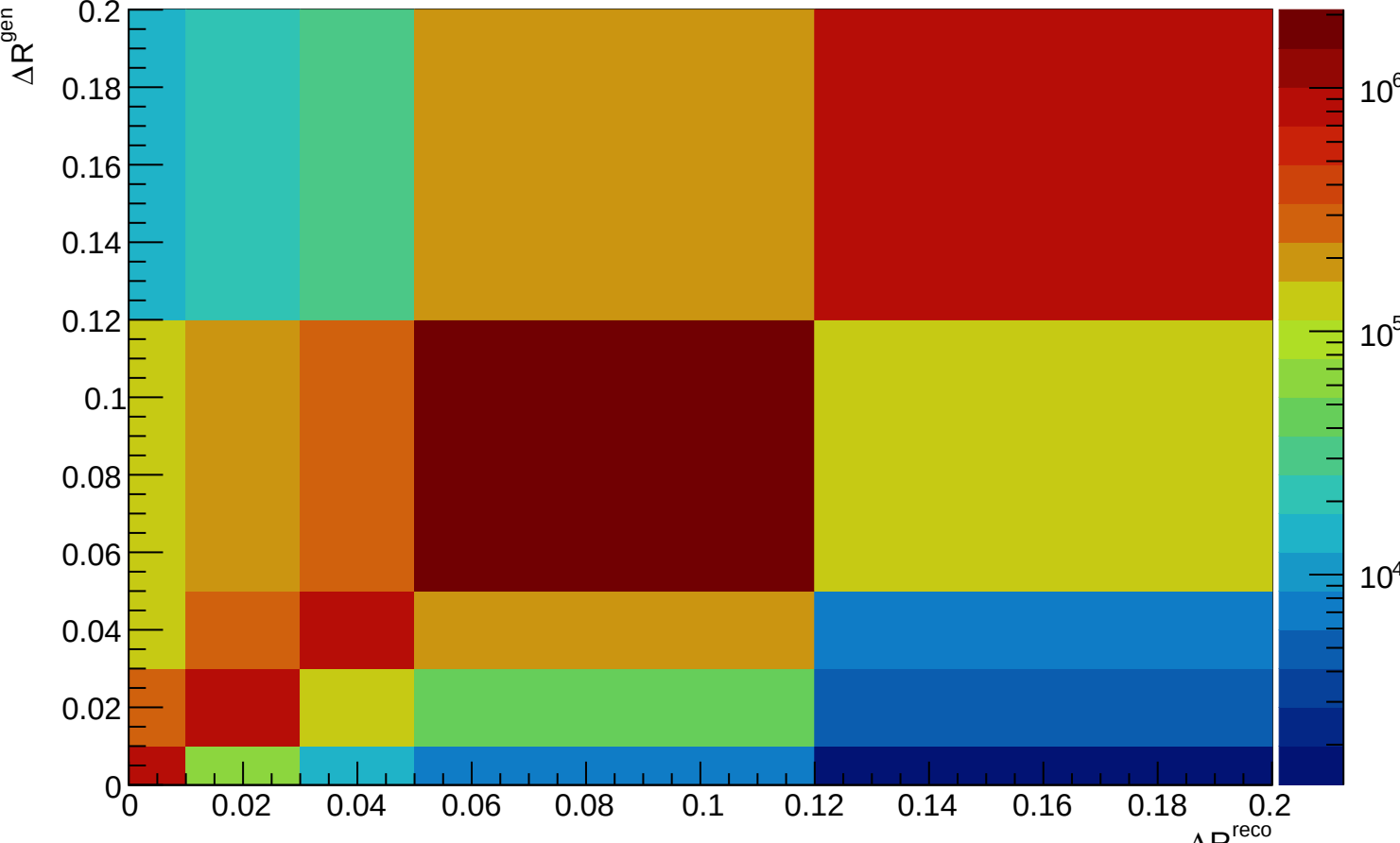
Response matrix projection on \Delta R
