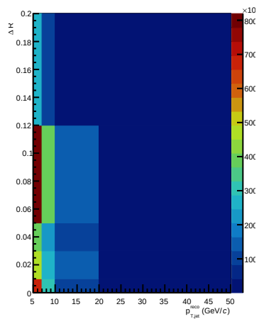
Fed-down with e_{kin}^{detector} correction
