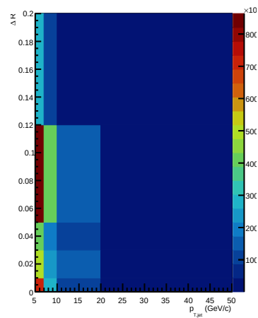
Background subtracted, efficiency corrected, fed down data distribution
