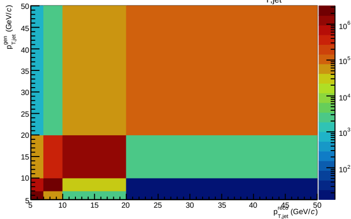
Response matrix projection on p_{T,\text{jet}}
