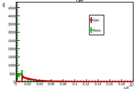
Migration entries p_{T,\text{jet}} \in [10,20]\text{GeV}/c
