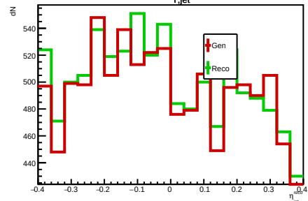
Migration entries p_{T,\text{jet}} \in [10,20]\text{GeV}/c
