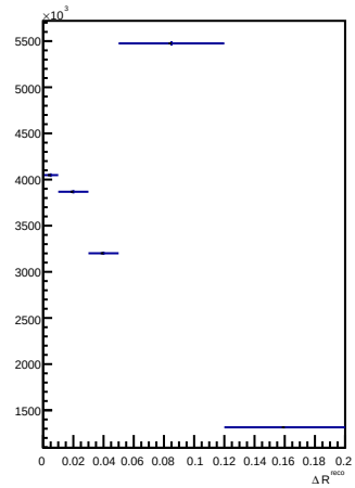
Fed-down with e_{kin}^{detector} correction
