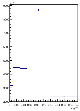
Unfolded with e_{kin}^{particle} correction with 8 iterations
