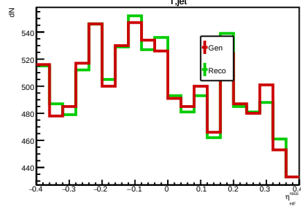
Migration entries p_{T,\text{jet}} \in [10,20]\text{GeV}/c
