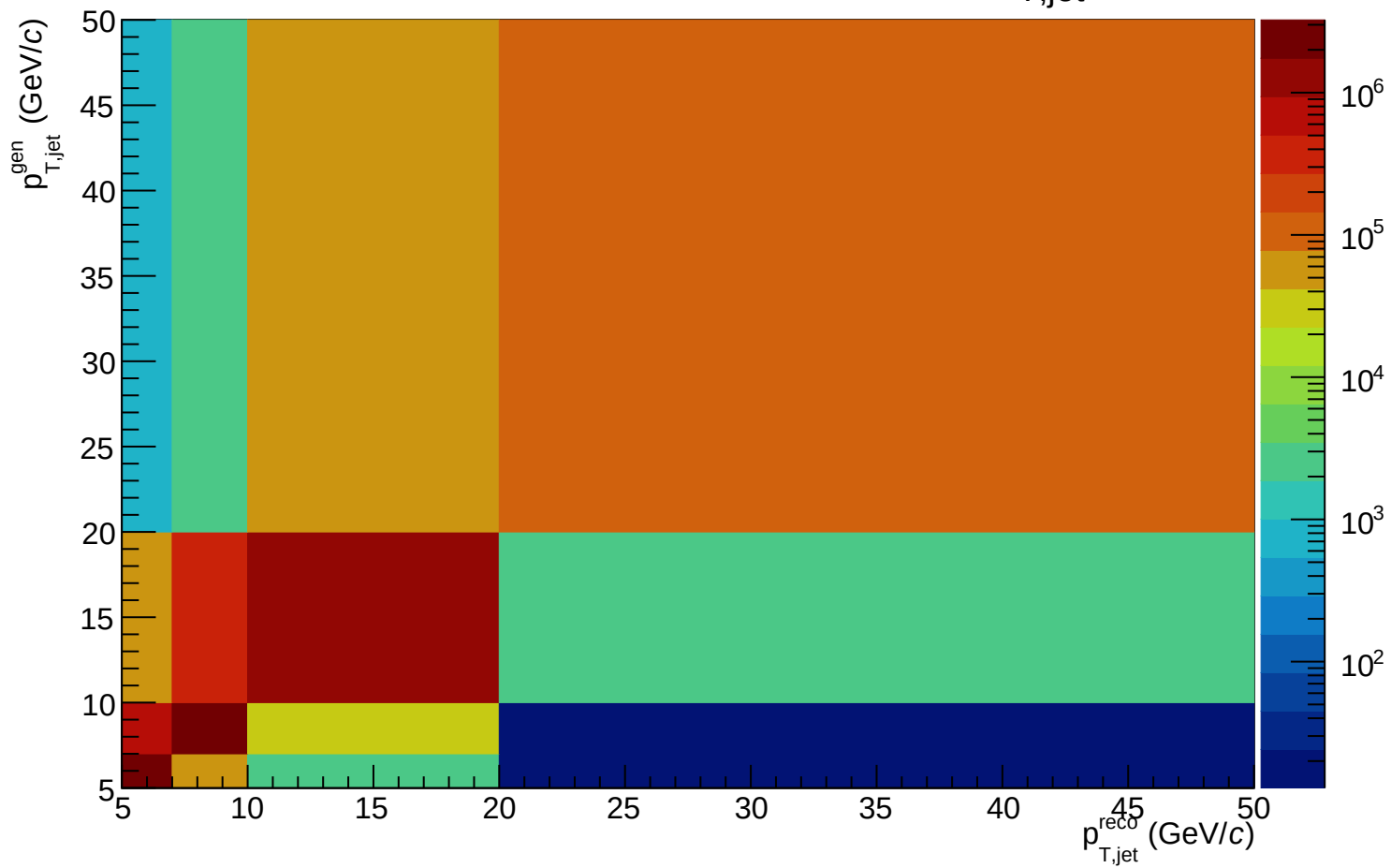
Response matrix projection on p_{T,\text{jet}}
