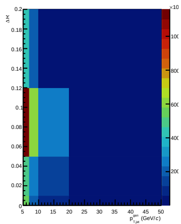
Unfolded with e_{kin}^{particle} correction with 8 iterations
