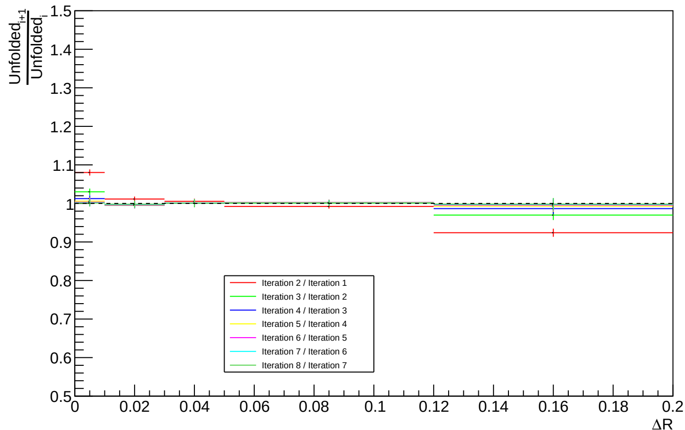
Consecutive ratios of unfolded distributions with different # of iterations
