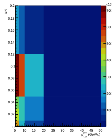
Immediately unfolded 2D histogram with 8 iterations
