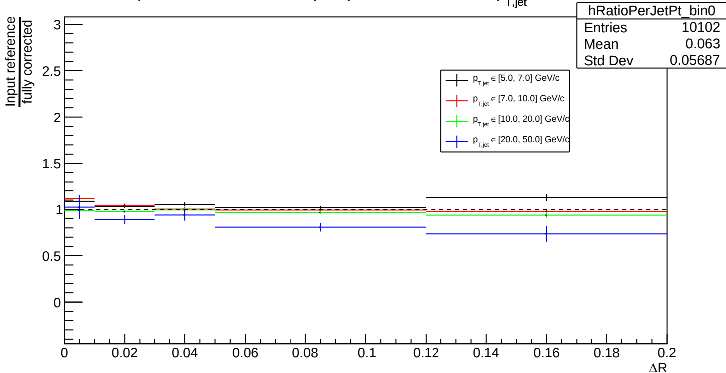
Input distribution divided by fully corrected for each p_{T,jet} bin GeV/c
