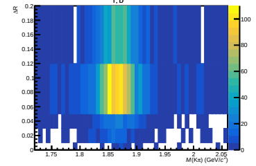
10 < p_{T, D^0} < 12 GeV/c
