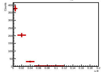
Side-band subtracted histogram for 16.0 < p_{T, \ell^*} < 20.0 GeV/c
