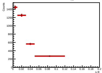
Side-band subtracted histogram for 12.0 < p_{T, \ell^*} < 16.0 GeV/c
