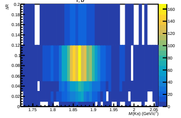
16 < p_{T, D^0} < 20 GeV/c
