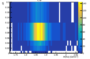
12 < p_{T, D^0} < 16 GeV/c
