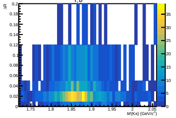
16 < p_{T, D^0} < 20 GeV/c
