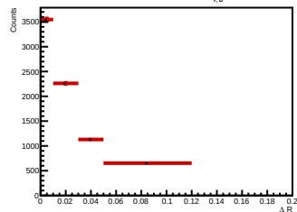
Side-band subtracted histogram for 7.0 < p_{T,d^*} < 8.0 GeV/c
