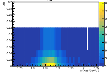
16 < p_{T, D^0} < 20 \text{ GeV}/c (Fit failed)
