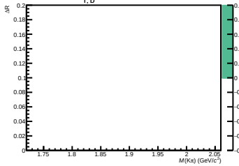
12 < p_{T, D^0} < 16 \text{ GeV}/c (Fit failed)
