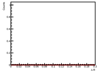
Side-band subtracted histogram for 1.0 < p_{T,d^*} < 2.0 GeV/c
