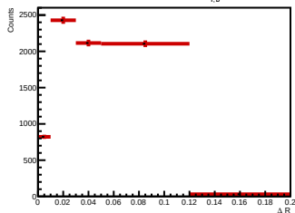
Side-band subtracted histogram for 6.0 < p_{T,d^*} < 7.0 GeV/c
