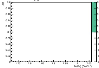
6 < p_{T, D^0} < 7 \text{ GeV}/c
