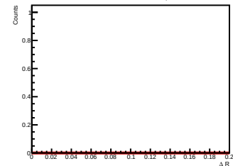
Side-band subtracted histogram for 16.0 < p_{T,d^*} < 20.0 GeV/c
