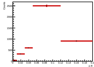
Side-band subtracted histogram for 4.0 < p_{T,d^*} < 5.0 GeV/c
