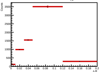
Side-band subtracted histogram for 5.0 < p_{T,d^*} < 6.0 GeV/c
