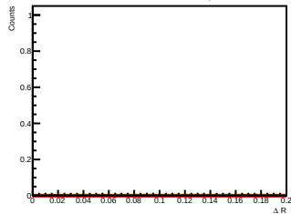
Side-band subtracted histogram for 2.0 < p_{T,d^*} < 3.0 GeV/c
