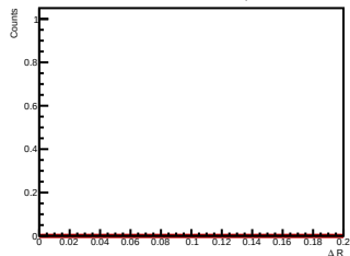
Side-band subtracted histogram for 10.0 < p_{T,d^*} < 12.0 GeV/c
