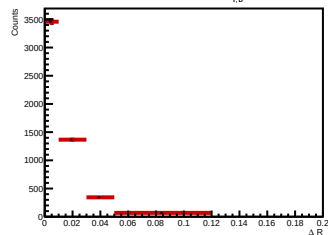
Side-band subtracted histogram for 8.0 < p_{T,d^*} < 10.0 GeV/c
