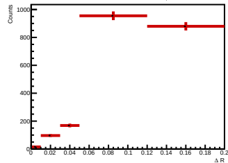
Side-band subtracted histogram for 3.0 < p_{T,d^*} < 4.0 GeV/c
