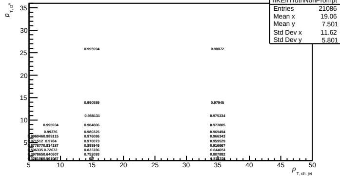
\epsilon_{\text{kinematic}} of particle level non-prompt D^0
