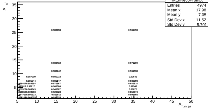
\epsilon_{\text{kinematic}} of detector level prompt D^0
