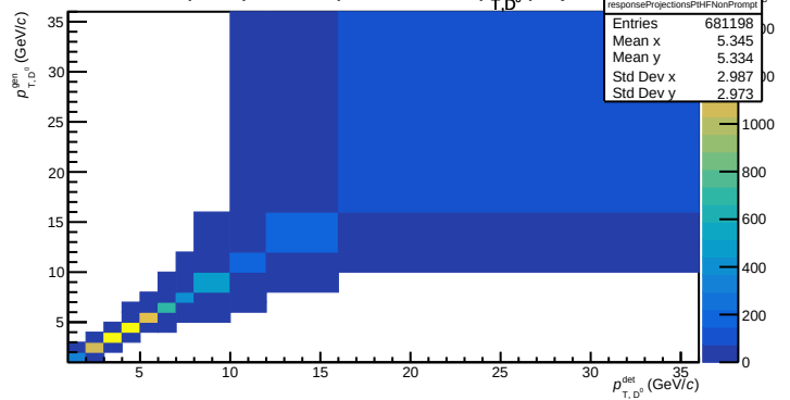
Non-prompt D^0 's reponse matrix p_{T, D^0} projection
