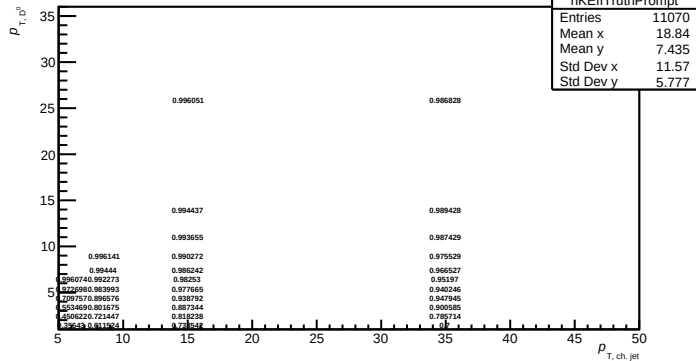
\epsilon_{\text{kinematic}} of particle level prompt D^0
