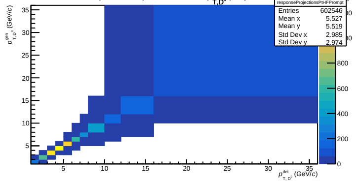
Prompt D^0 's reponse matrix p_{T, D^0} projection
