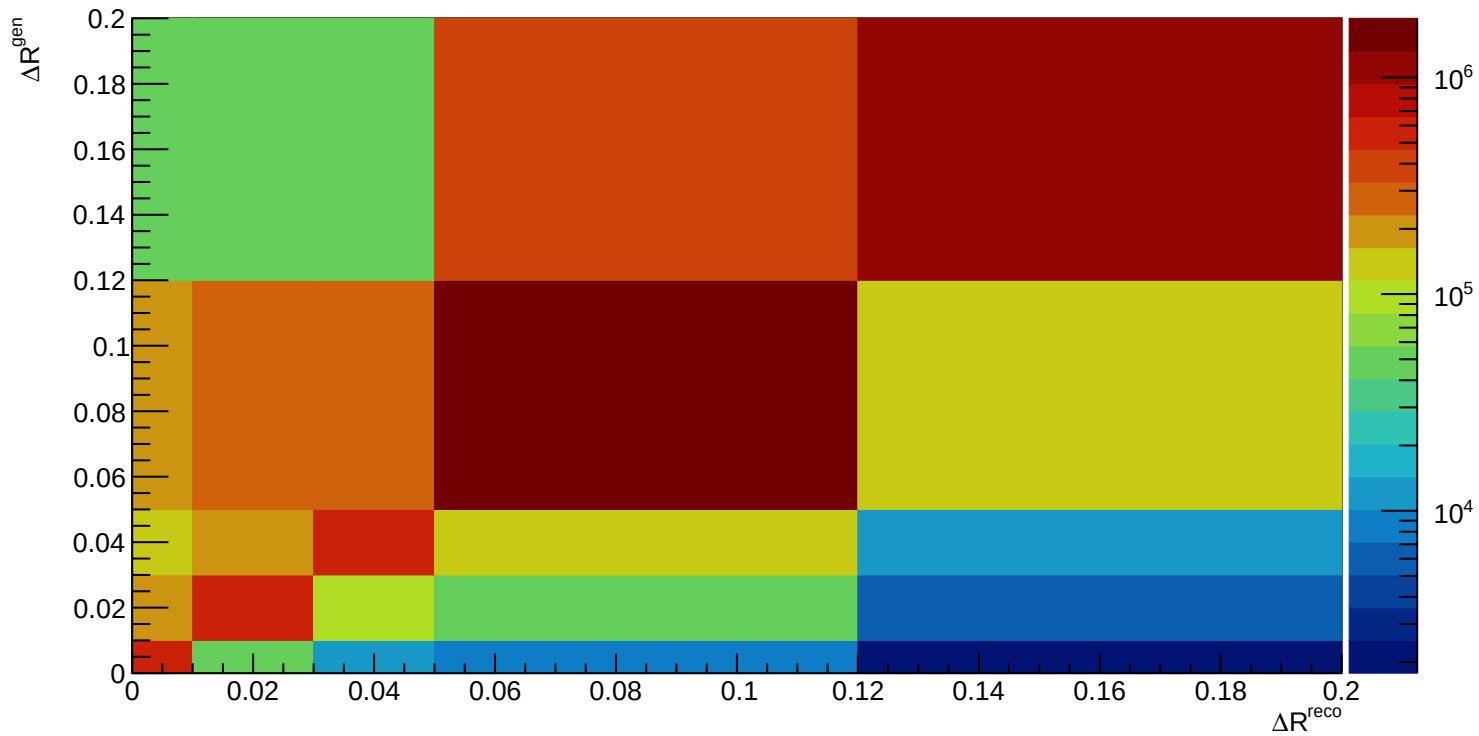
Response matrix \Delta R projection
