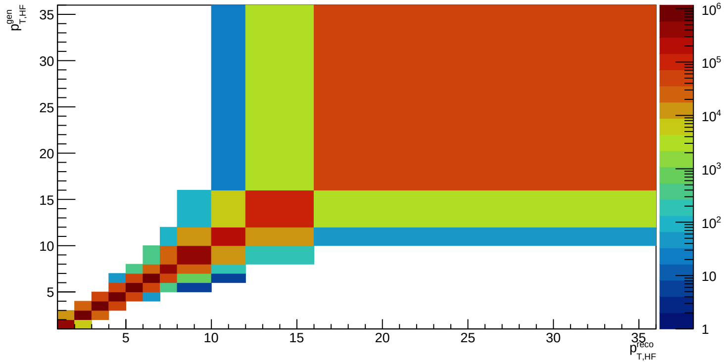
Response matrix p_{T,HF} projection
