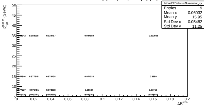
Detector level kinematic efficiency (non-prompt D^0 's) xy projection
