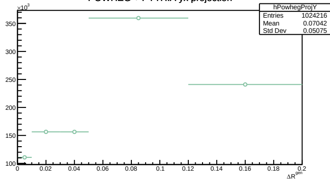
POWHEG + PYTHIA yx projection
