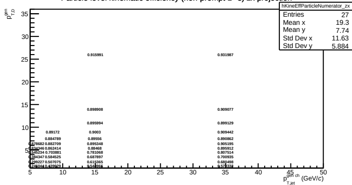
Particle level kinematic efficiency (non-prompt D^0 s) zx projection
