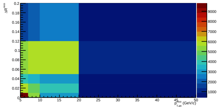
Folded 2D histogram with \epsilon_{kin}^{detector} correction yx projection
