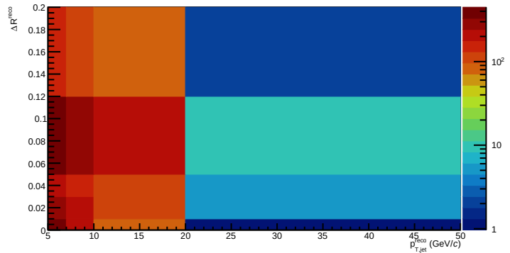
Pure non-prompt fully corrected distribution (as found in data)
