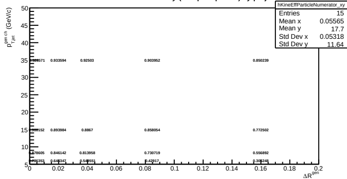
Particle level kinematic efficiency (non-prompt D^0 s) xy projection
