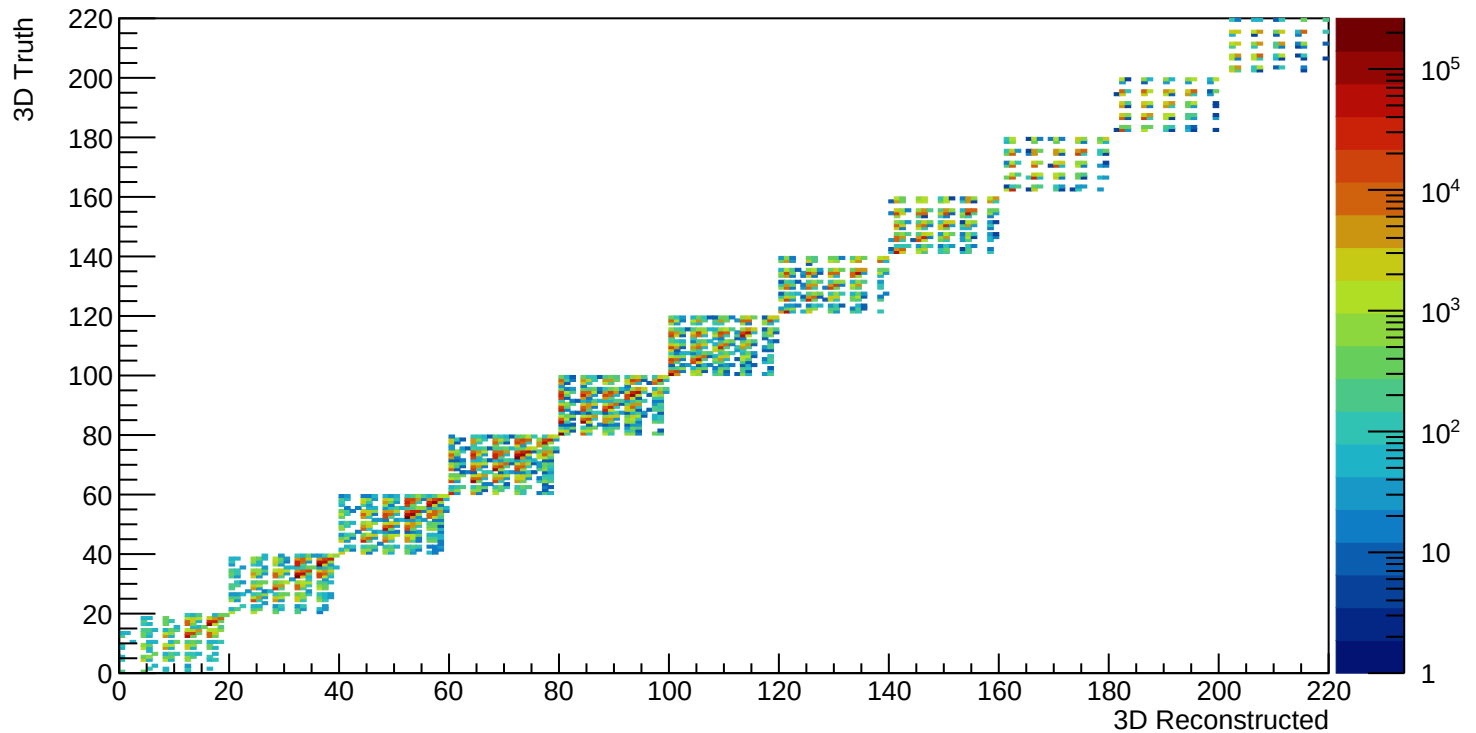
2D response matrix from 6D RooUnfoldResponse - non-prompt D^0 's
