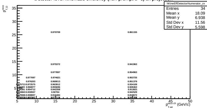
Detector level kinematic efficiency (non-prompt D^0 's) zx projection
