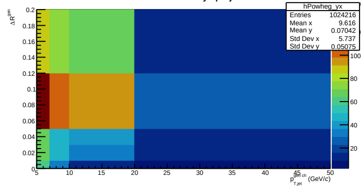
POWHEG + PYTHIA yx projection
