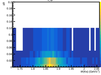
12 < p_{T, D^0} < 16 GeV/c
