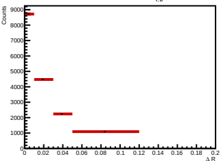
Side-band subtracted histogram for 5.0 < p_{T, \phi^*} < 6.0 GeV/c
