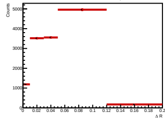
Side-band subtracted histogram for 4.0 < p_{T, \phi^*} < 5.0 GeV/c
