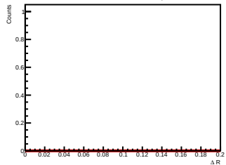
Side-band subtracted histogram for 1.0 < p_{T, \phi^*} < 2.0 GeV/c
