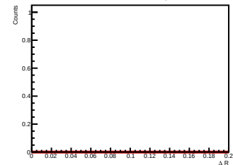
Side-band subtracted histogram for 16.0 < p_{T,d^*} < 36.0 GeV/c
