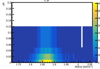
16 < p_{T, D^0} < 36 \text{ GeV}/c (Fit failed)
