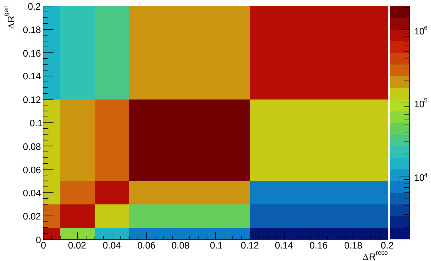
Response matrix projection on \Delta R
