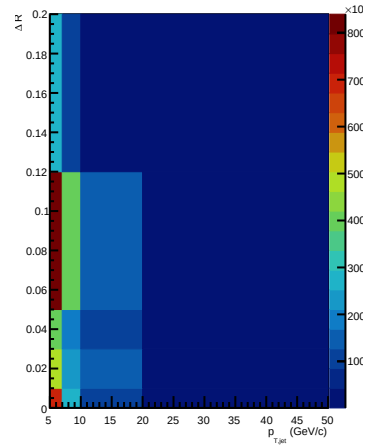
Background subtracted, efficiency corrected, test down data distribution
