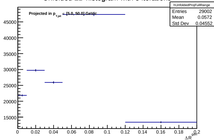
Unfolded 2D histogram with 8 iterations
