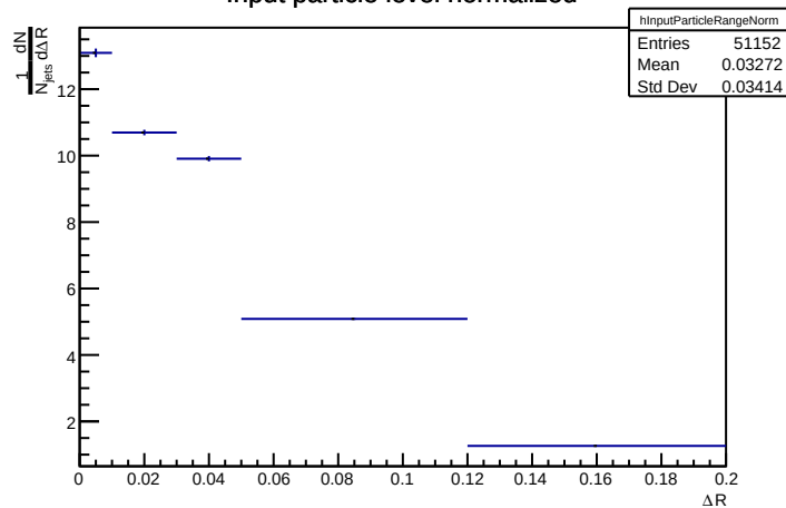
Input particle level normalized
