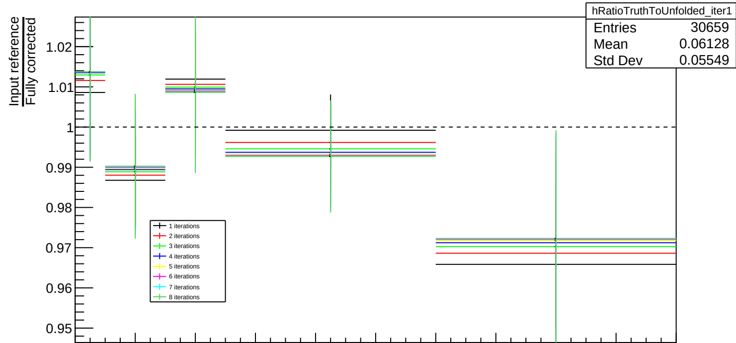
Ratio of input particle level to unfolded distribution, for each iteration
