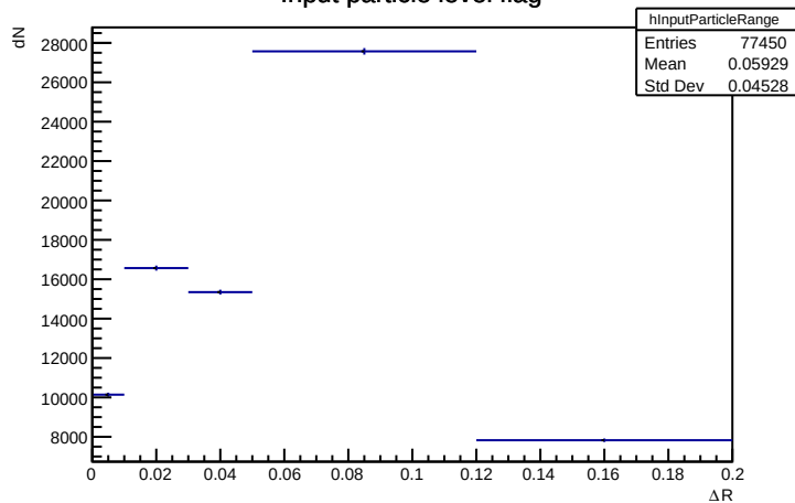
Input particle level flag
