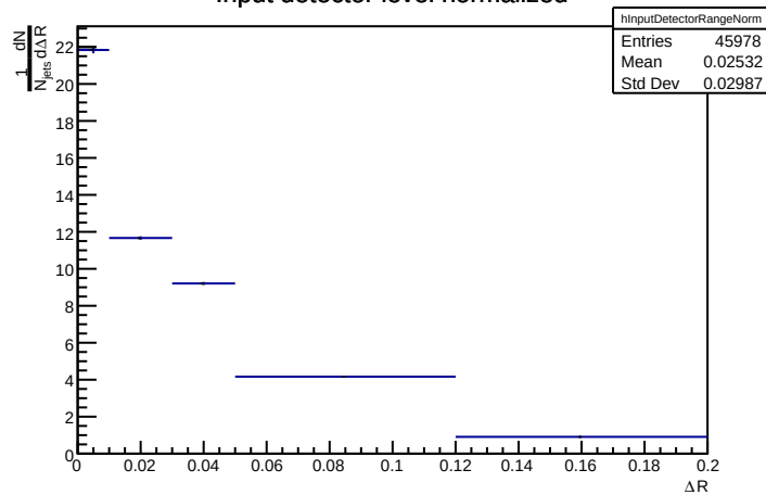
Input detector level normalized
