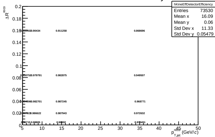
Detector level kinematic efficiency
