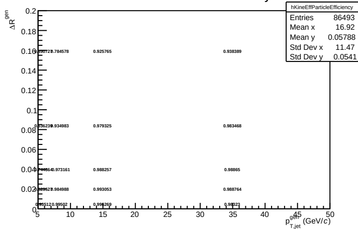
Particle level kinematic efficiency
