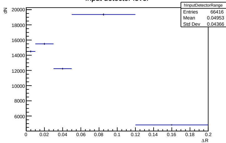
Input detector level
