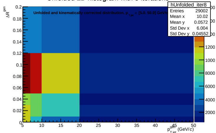
Unfolded 2D histogram with 8 iterations
