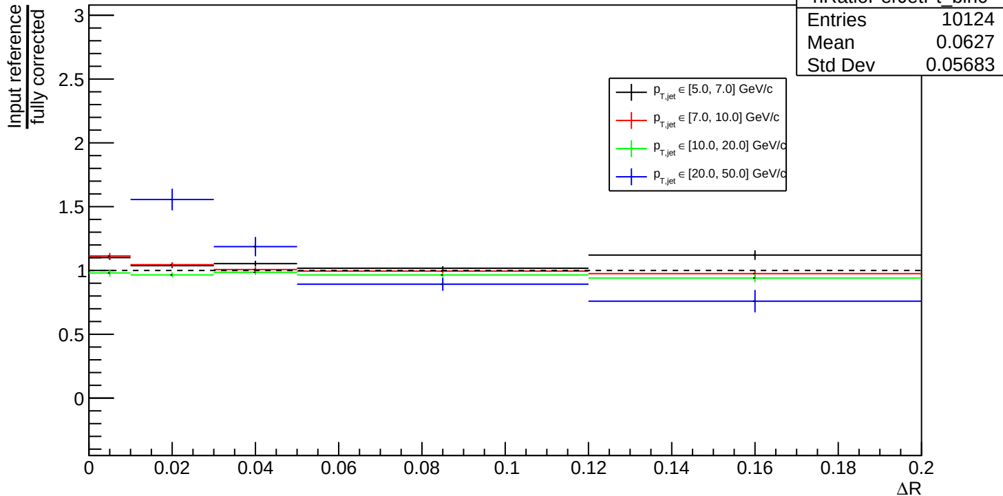
Input distribution divided by fully corrected for each p_{T,jet} bin GeV/c
