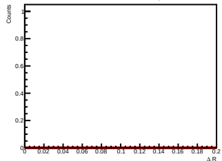
Side-band subtracted histogram for 1.0 < p_{T,0^+} < 2.0 GeV/c
