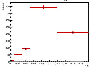
Side-band subtracted histogram for 5.0 < p_{T,0^+} < 6.0 GeV/c
