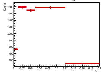
Side-band subtracted histogram for 8.0 < p_{T,0^+} < 10.0 GeV/c
