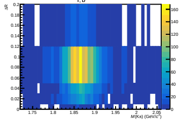
16 < p_{T, D^0} < 36 \text{ GeV}/c
