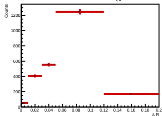
Side-band subtracted histogram for 7.0 < p_{T,0^+} < 8.0 GeV/c
