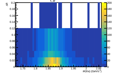
10 < p_{T, D^0} < 12 \text{ GeV}/c
