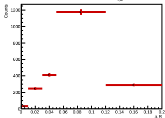
Side-band subtracted histogram for 6.0 < p_{T,0^+} < 7.0 GeV/c
