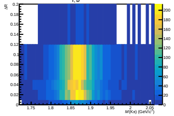
8 < p_{T, D^0} < 10 \text{ GeV}/c
