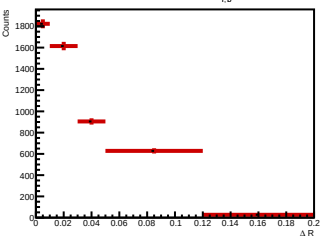
Side-band subtracted histogram for 10.0 < p_{T,0^+} < 12.0 GeV/c
