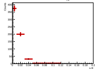
Side-band subtracted histogram for 16.0 < p_{T,0^+} < 36.0 GeV/c
