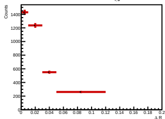
Side-band subtracted histogram for 12.0 < p_{T,0^+} < 16.0 GeV/c
