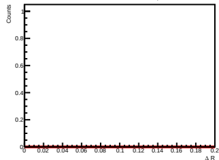
Side-band subtracted histogram for 3.0 < p_{T,0^+} < 4.0 GeV/c
