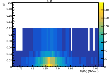
12 < p_{T, D^0} < 16 \text{ GeV}/c
