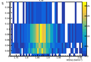
12 < p_{T, D^0} < 16 GeV/c
