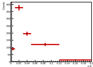
Side-band subtracted histogram for 16.0 < p_{T, D^0} < 36.0 GeV/c
