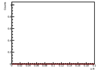
Side-band subtracted histogram for 4.0 < p_{T, D^0} < 5.0 GeV/c
