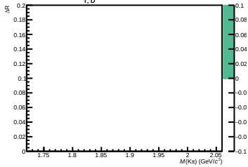
10 < p_{T, D^0} < 12 GeV/c (Fit failed)
