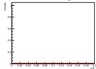
Side-band subtracted histogram for 8.0 < p_{T, D^0} < 10.0 GeV/c
