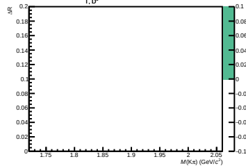
8 < p_{T, D^0} < 10 GeV/c (Fit failed)
