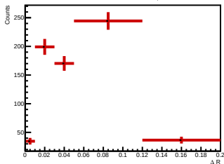
Side-band subtracted histogram for 12.0 < p_{T, D^0} < 16.0 GeV/c
