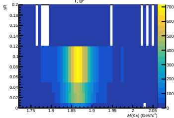
4 < p_{T, D^0} < 5 \text{ GeV}/c
