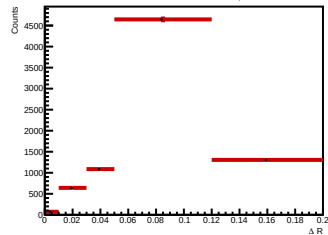
Side-band subtracted histogram for 3.0 < p_{T, \phi^0} < 4.0 GeV/c
