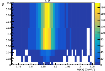
2 < p_{T, D^0} < 3 \text{ GeV}/c
