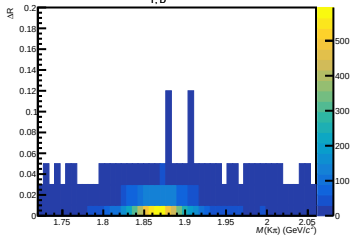
6 < p_{T, D^0} < 7 \text{ GeV}/c
