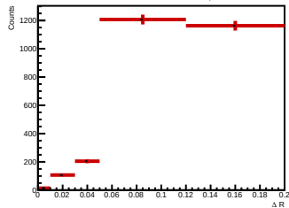
Side-band subtracted histogram for 2.0 < p_{T, \phi^0} < 3.0 GeV/c
