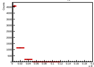
Side-band subtracted histogram for 6.0 < p_{T, \phi^0} < 7.0 GeV/c
