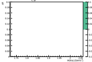
10 < p_{T, D^0} < 12 \text{ GeV}/c (Fit failed)
