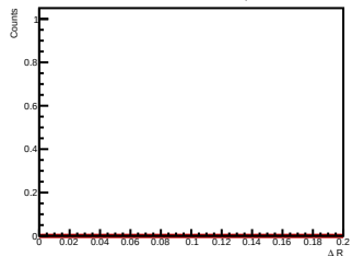
Side-band subtracted histogram for 10.0 < p_{T, \phi^0} < 12.0 GeV/c
