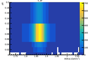
3 < p_{T, D^0} < 4 \text{ GeV}/c
