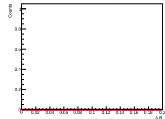
Side-band subtracted histogram for 12.0 < p_{T, \phi^0} < 16.0 GeV/c
