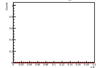
Side-band subtracted histogram for 8.0 < p_{T, \phi^0} < 10.0 GeV/c
