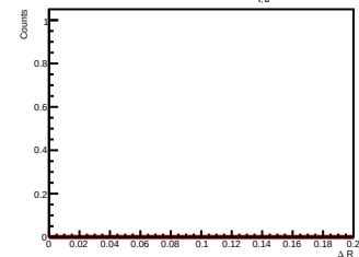
Side-band subtracted histogram for 7.0 < p_{T, \phi^0} < 8.0 GeV/c
