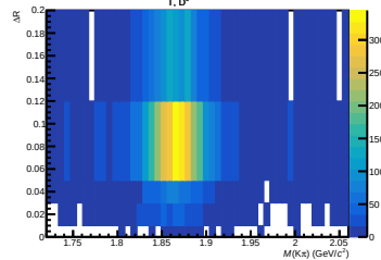
8 < p_{T, D^0} < 10 \text{ GeV}/c
