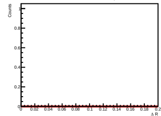
Side-band subtracted histogram for 16.0 < p_{T,d^*} < 36.0 GeV/c
