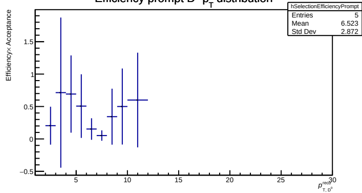
Efficiency prompt D^0 p_T distribution
