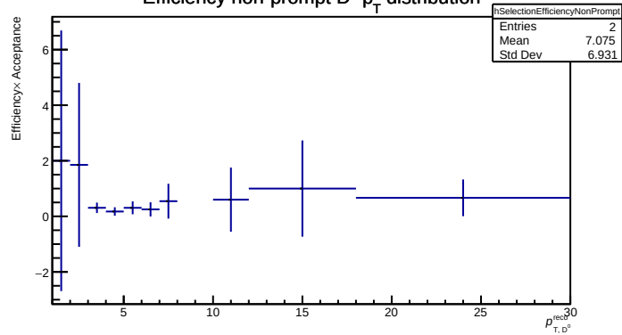
Efficiency non-prompt D^0 p_T distribution
