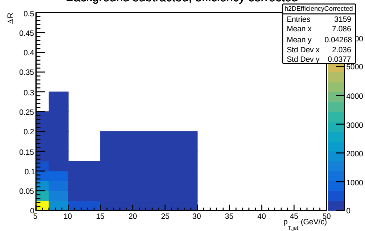
Background subtracted, efficiency corrected
