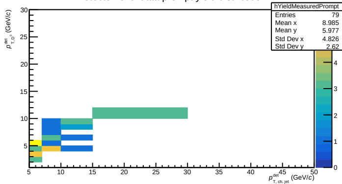
Detector level data prompt yield distribution
