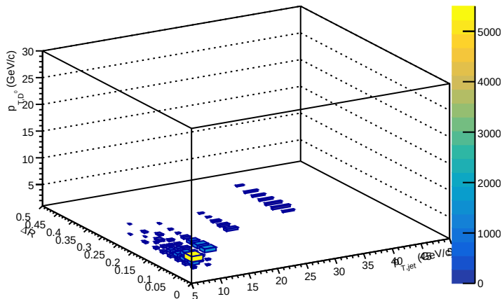
Background subtracted, efficiency corrected
