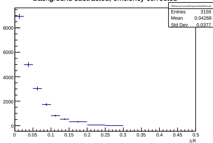
Background subtracted, efficiency corrected
