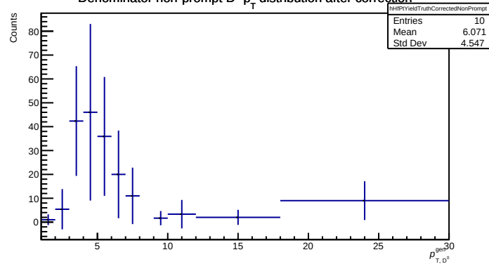
Denominator non-prompt D^0 p_T distribution after correction
