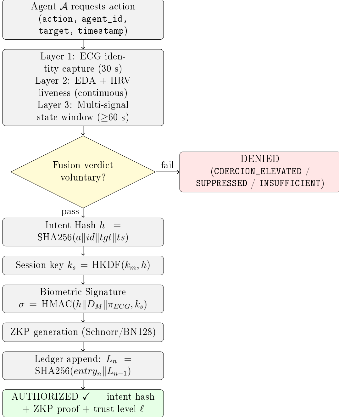
Figure 1: LICET v2 authorization flow with three-layer physiological verification.
