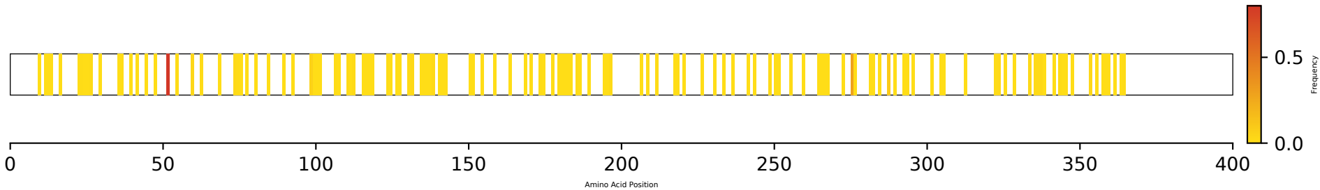
Nonsynonymous Mutation Density
