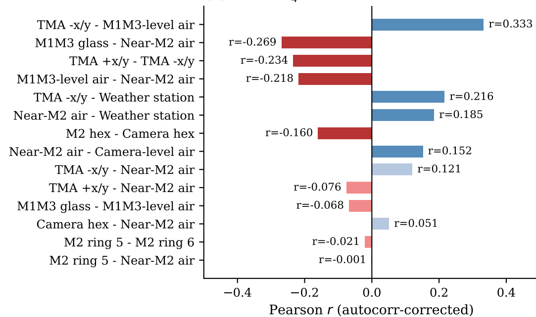
(b) \Delta T vs z_4^{(c)}
