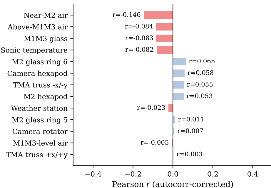
(c) dT/dt vs dz_4/dt
