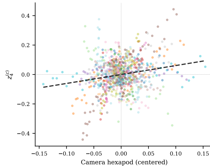
Camera hexapod r = 0.204
