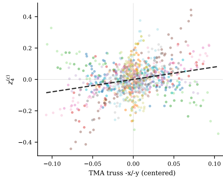
TMA truss -x/-y r = 0.255
