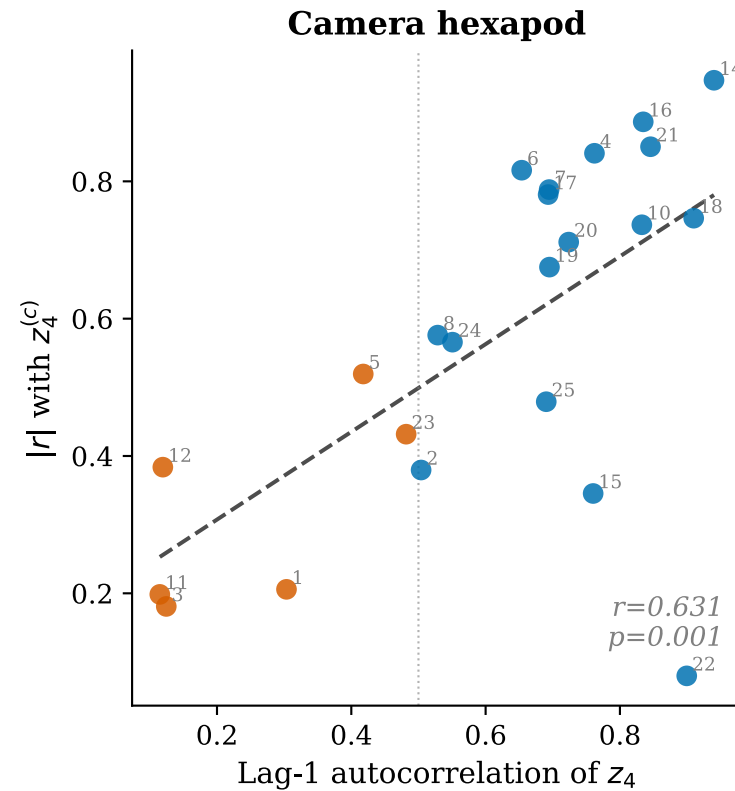
Per-run |r| vs smoothness (lag-1 autocorr) — top 5 sensors Blue = smooth (high autocorr) Orange = dynamic Dotted = threshold
