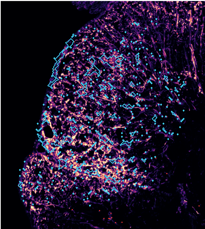
weak border · C_L_3 (MILD30) border vimentin -0.26 z · depth 561 μm · escape +1.70
