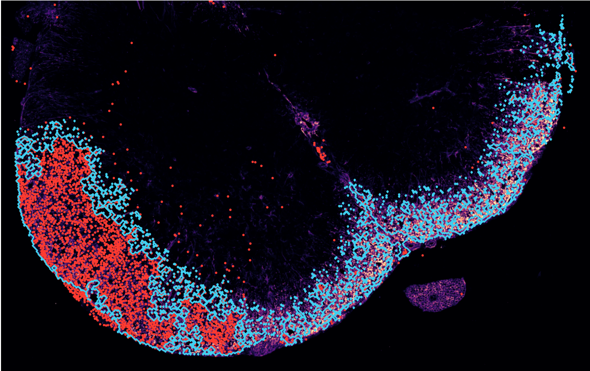
strong border · C_L_3 (MILD30) border vimentin +4.93 z · depth 152 μm · escape +3.75
