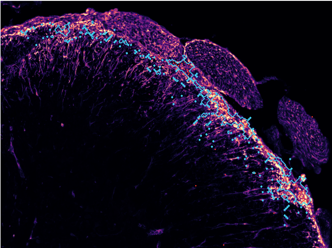
strong border · RR_MP_4 (MONOPHASIC) border vimentin +7.23 z · depth 119 μm · escape +2.74
