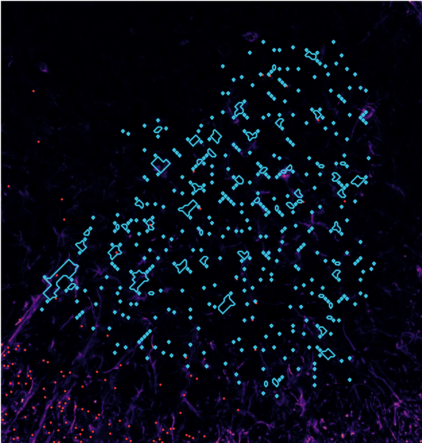
weak border · C_L_3 (MILD30) border vimentin -0.26 z · depth 561 μm · escape +1.70
