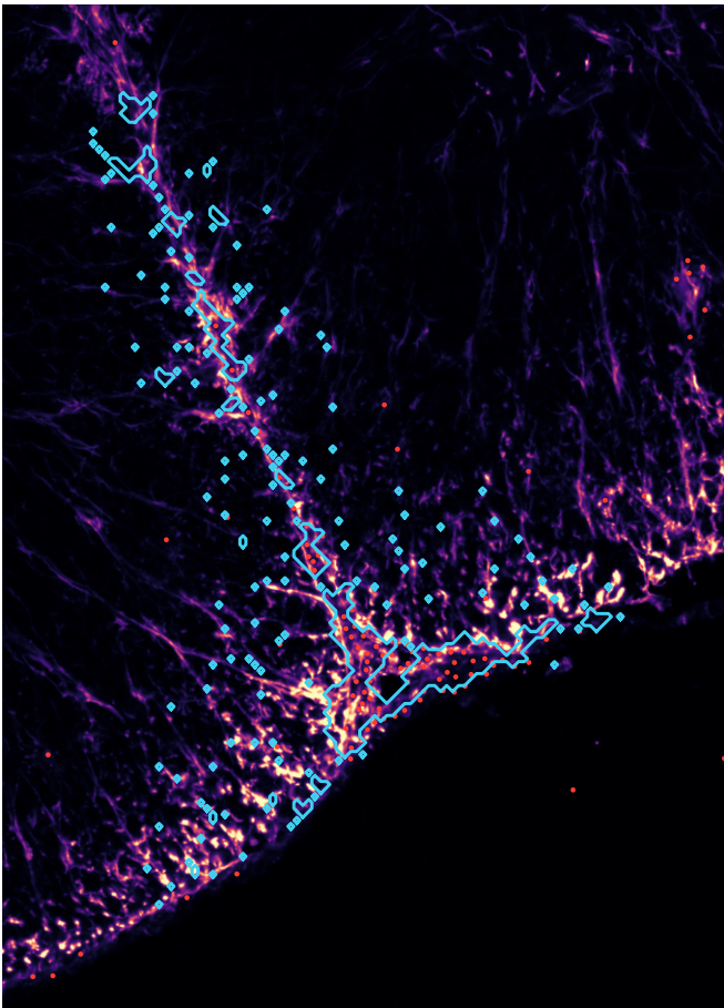
weak border · C_L_4 (MILD30) border vimentin +0.59 z · depth 199 μm · escape +4.00
